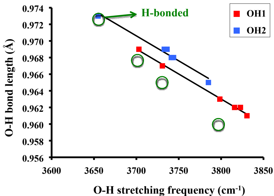
Fig. 7 Plot of O-H bond length as a function of the vibrational frequency of the O-H bond for the various conformers (A-G) of lactic acid using B3LYP-D3/aug-cc-pVTZ.
