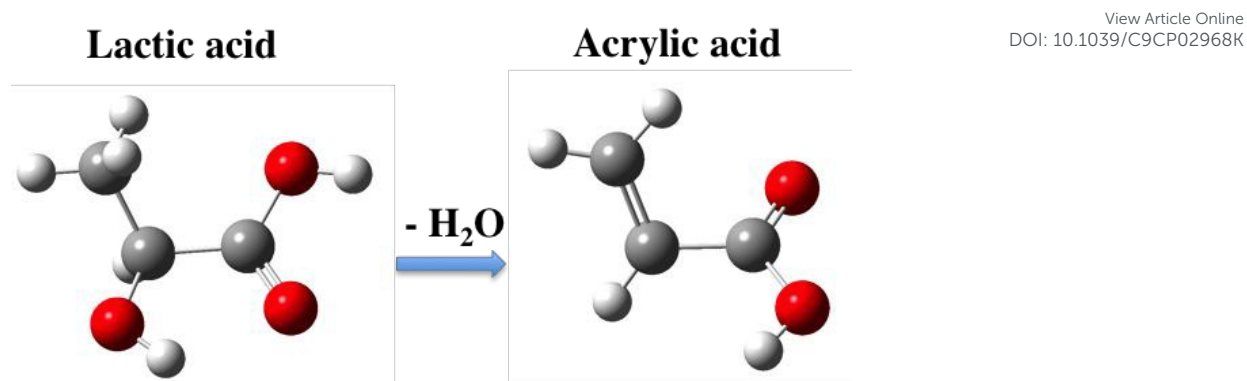
Figure 1. Figure showing the dehydration of lactic acid to acrylic acid
