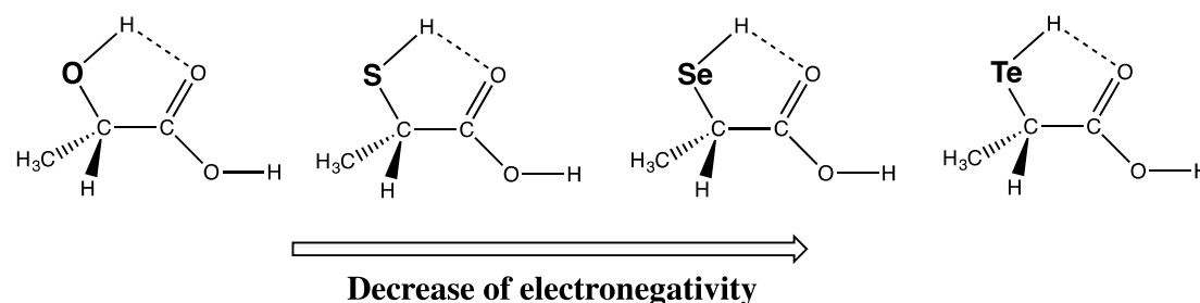
Figure 4. Various lactic acid-like compounds examined for the formation of an intra-molecular H-bond
