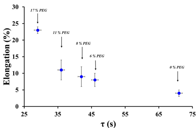
Fig. 10. A plot of the relationship between tensile elongation and molecular relaxation time ( \tau ) for the HPMC-PEG films.
