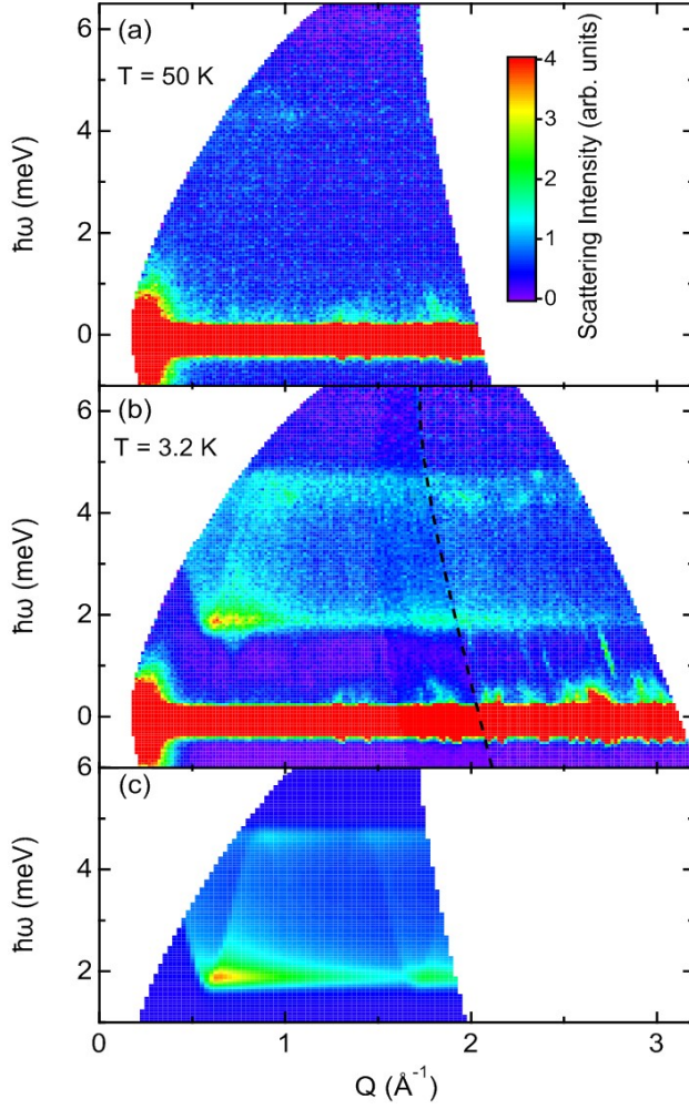
FIG. 2. (a), (b) Color contour plots of the E_i = 7.5 meV HYSPEC data for \text{AgVOAsO}_4 at T = 50 K and T = 3.2 K. A gapped magnetic excitation spectrum is clearly visible in the low-temperature data. The data to the left of the black dashed line in (b) was collected using a single orientation for the HYSPEC detector bank. (c) Color contour plot for the alternating chain model described in the text with best fit parameters J = 3.43(7) meV and J' = 2.25(9) meV. The INS data was only fit over the Q - \hbar\omega region presented in this figure.
