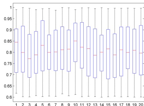
Figure 6(d): Percentage of EF per generation replication2
