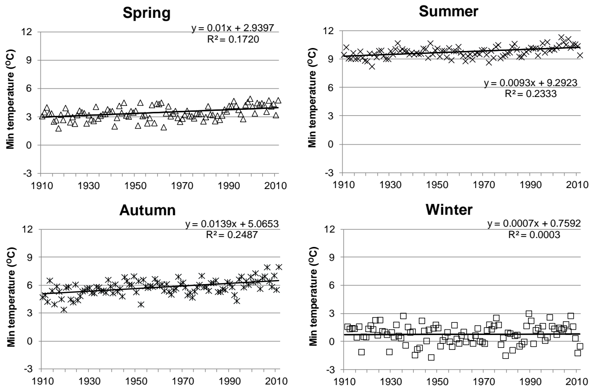
Appendix Figure 2. UK mean seasonal minimum temperatures (°C) 1910 – 2011 (x=1 for 1910).
