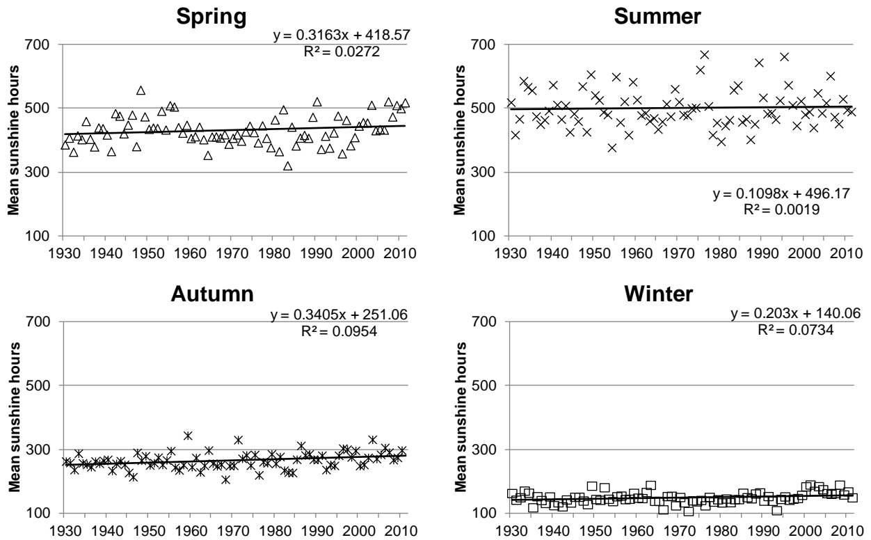
Appendix Figure 4. UK mean seasonal sunshine hours (totals) 1910 – 2011 ( x=1 for 1930).
