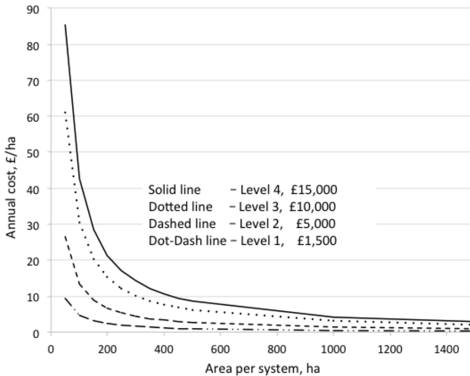
Figure 6. Annual cost ha -1 of the guidance system for four levels of capital expenditure.
