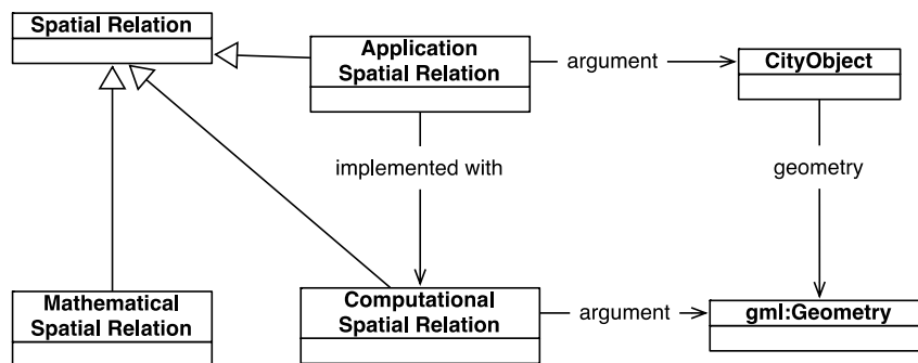
Fig. 16 Spatial Relations separated into 3 levels: Application, Computational and Mathematical.
