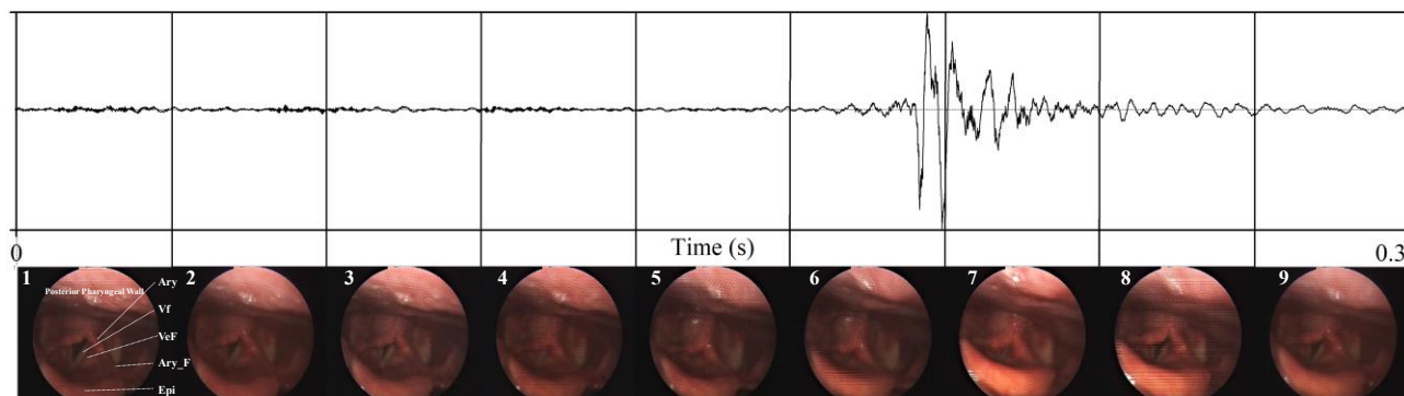
Figure 2: Acoustic waveform and its synchronized laryngoscopic images of an unaffricated classic kick-drum. Frame 1 to 3 show glottal adduction involving vocal folds and ventricular folds, frame 4 to 6 show supraglottal compression involving arytenoid cartilages and the aryepiglottic folds, frame 7 to 9 indicate glottal abduction involving vocal folds and ventricular folds (Frame 1: Vf = Vocal folds, VeF = Ventricular Folds, Ary = Arytenoids, Ary_F = aryepiglottic folds, Epi = Epiglottis).
