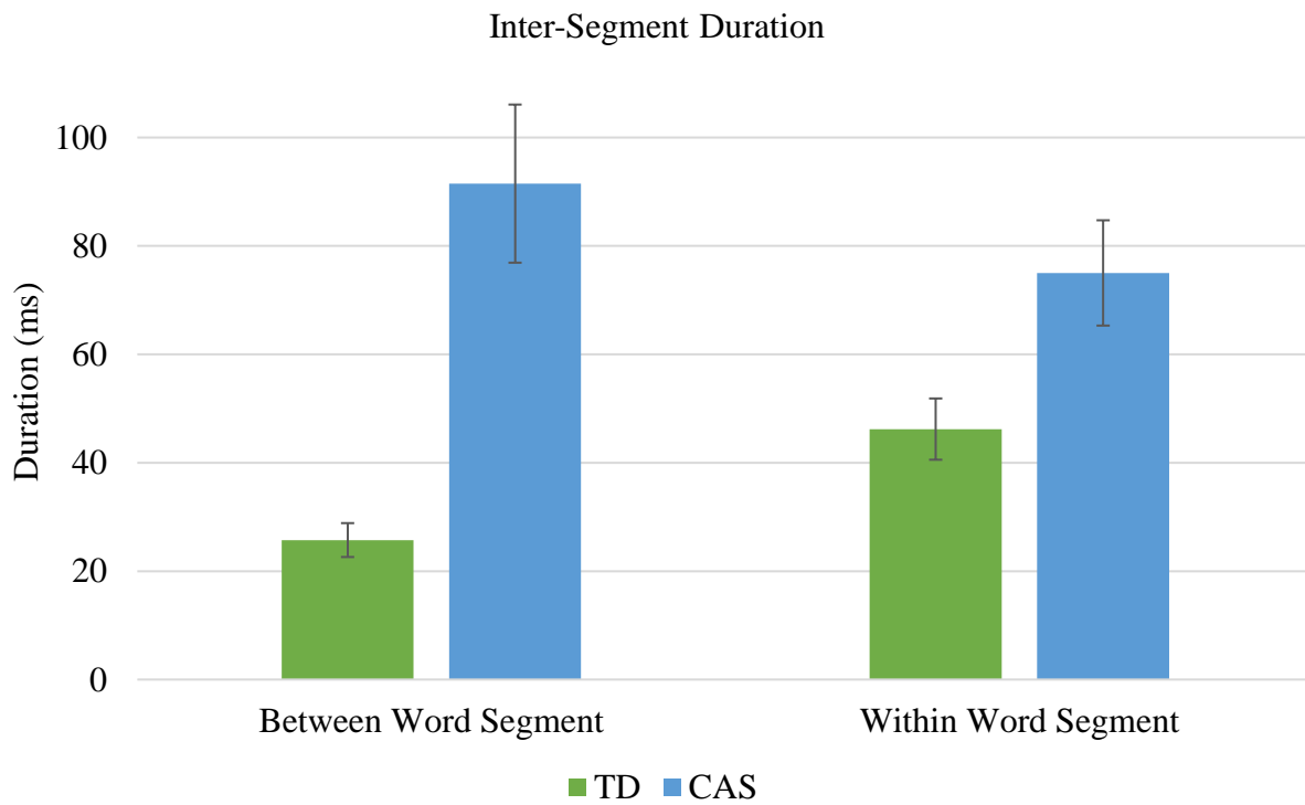
Figure 5. Comparison of inter-segment duration between and within words.
