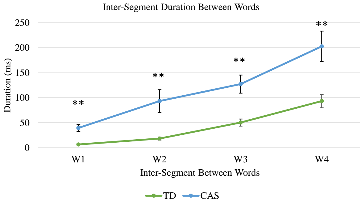
Figure 2. Inter-segment duration between words over the utterance.
