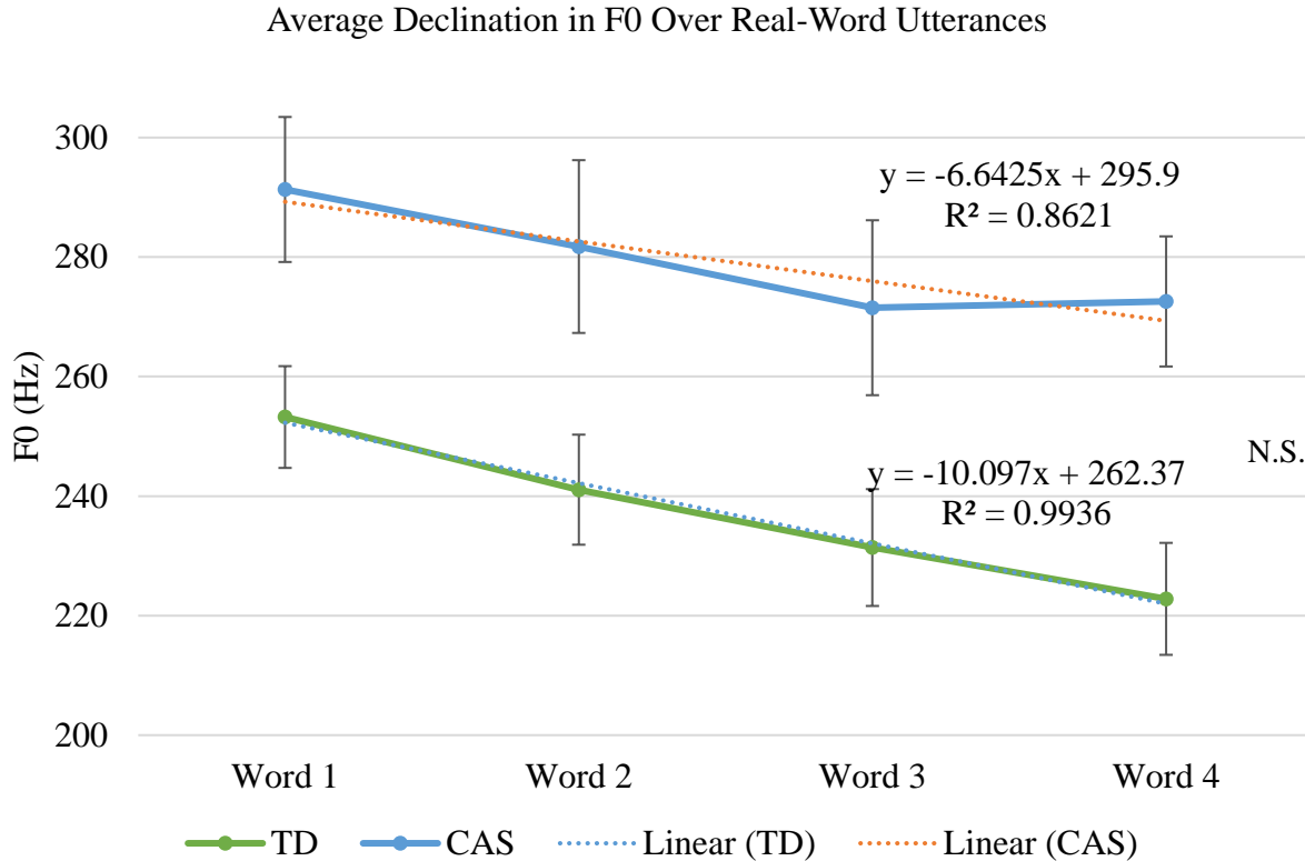
Figure 10. Average declination in F0 over real-word utterances.
