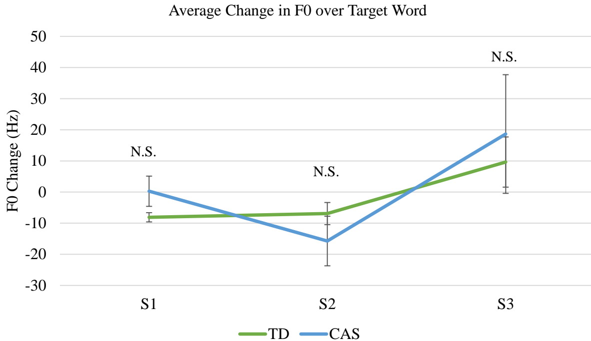
Figure 14. Average F0 differences between syllables within a target word for both groups.
