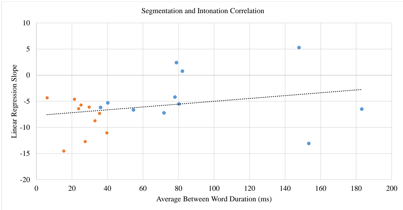
Figure 18. Pearson correlation depicting interaction between inter-segment duration between words and slope of the utterance related to F0 intonation. TD participants are represented in orange and CAS participants are represented in blue.
