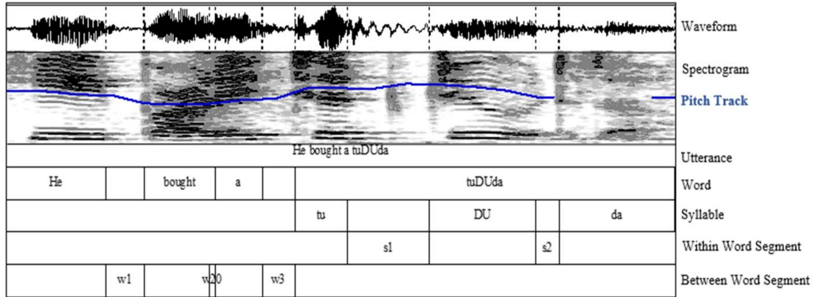
Figure 1. Praat coding example. Tier names indicated on the right reflect the type of data coded over the utterance. Interval barriers mark the start and end of each unit (utterance, word, syllable, or inter-segment). The blue line over the spectrogram indicates the F0/pitch track between the range of 50 and 500 Hz.
