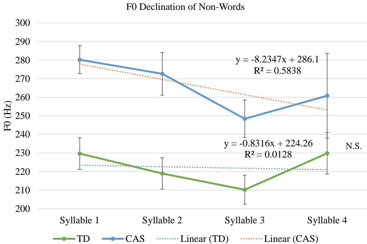
Figure 17. F0 declination of non-word target words for both groups.
