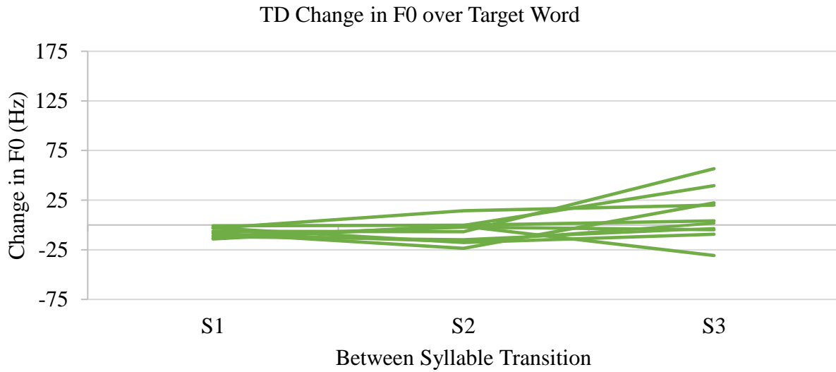
Figure 12. Participant F0 differences between syllables within a target word for TD population.
