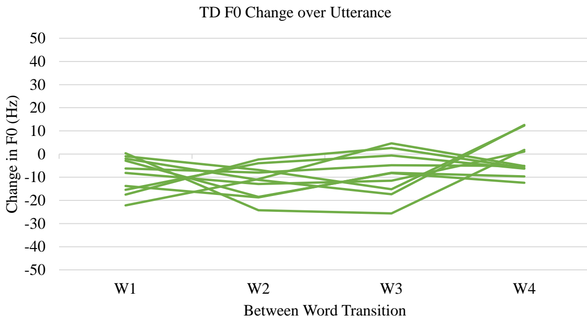
Figure 6. F0 differences between words within an utterance for TD population.
