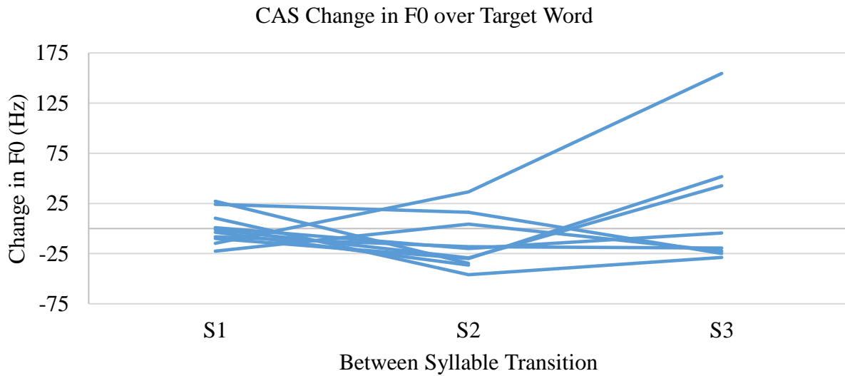
Figure 13. Participant F0 differences between syllables within a target word for CAS population.
