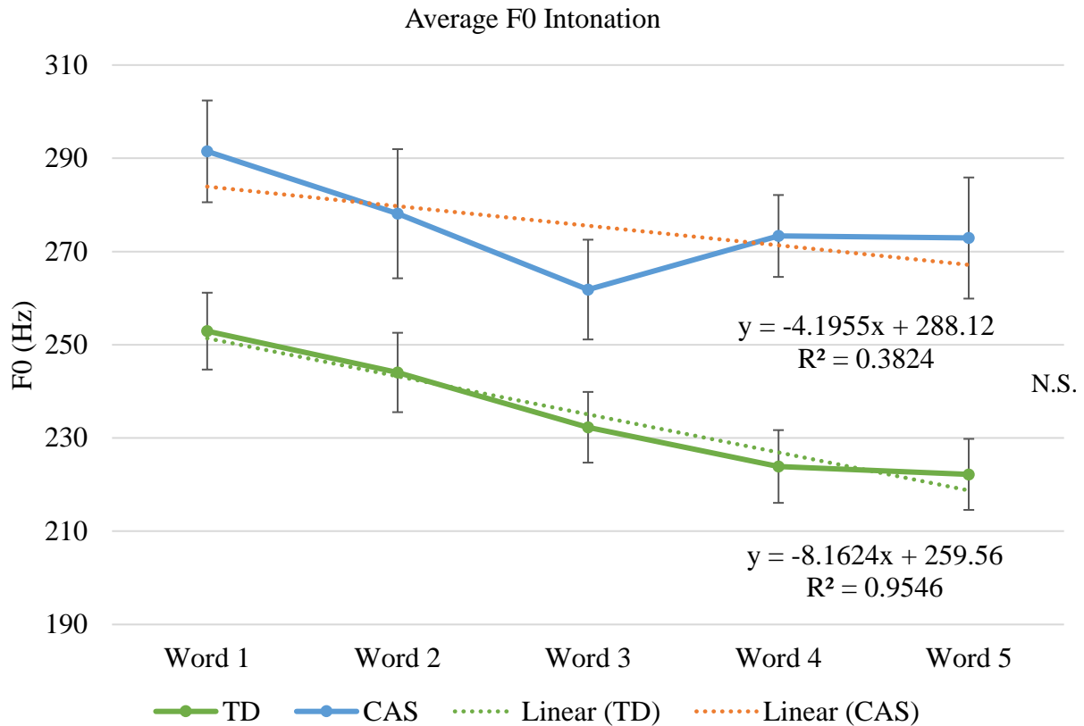
Figure 9. Average F0 intonation per word of the utterance for each group.
