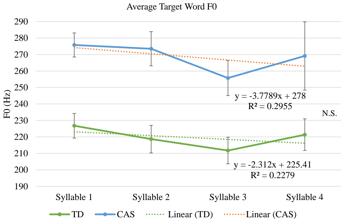
Figure 15. Average target word F0 per syllable in the word.
