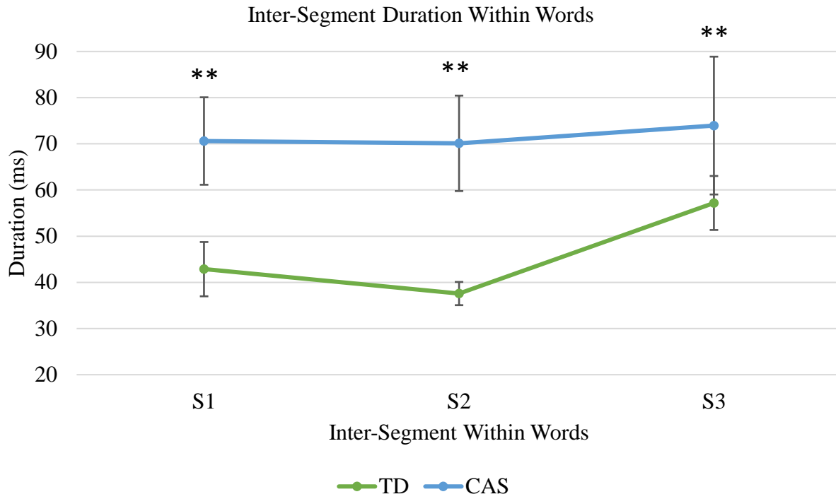
Figure 4. Inter-segment duration within words over the utterance.
