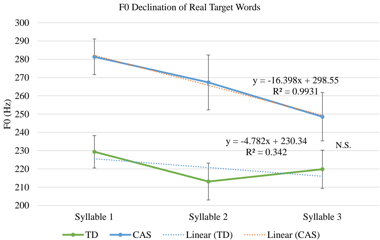
Figure 16. F0 declination of real target words for both groups.
