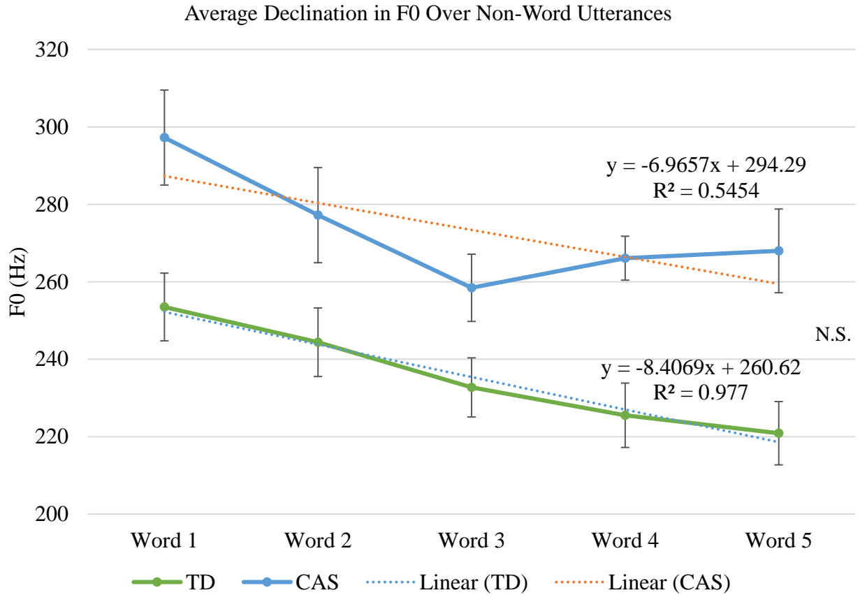
Figure 11. Average declination in F0 over non-word utterances for both groups.
