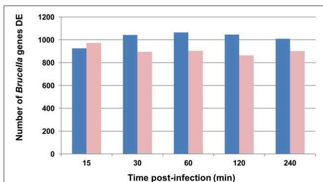
FIGURE 1 | Graphic representation of B. melitensis genes differentially expressed (DE) throughout the experiment. Blue bars represent genes activated; light red bars represent genes repressed. For differential analysis, the in vivo infected loop gene expression is compared to the in vitro log growth phase inoculum as the control.
