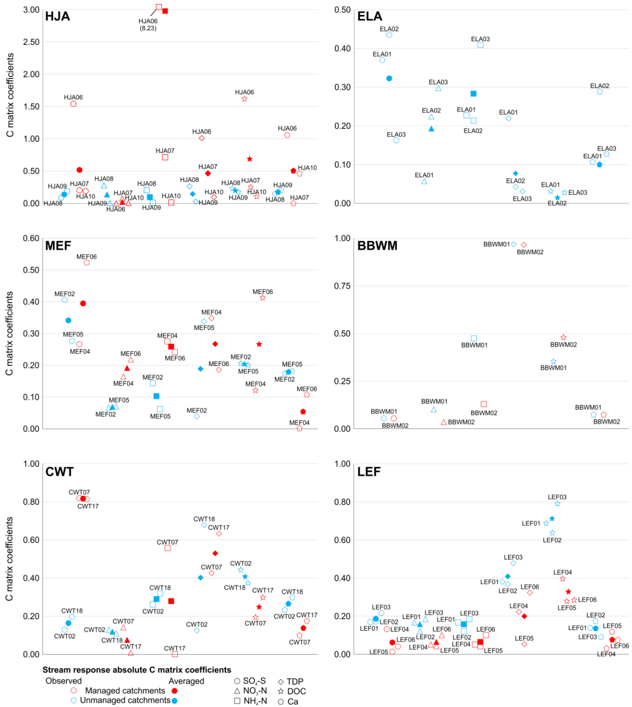
Figure 4.2 C matrix coefficients from best fitted global stressor models in all unmanaged and managed catchments at each site (note: axis scales are not standardized across all sites because the coefficient values are from different models). Larger C matrix coefficients indicate larger effects from the best fitted global stressor models. HJA was impacted by NO 3 -N deposition changes; ELA and MEF were impacted by air temperature changes. BBWM was impacted by NH 4 -N deposition changes; CWT was impacted by runoff changes; LEF was impacted by DIN deposition changes.
