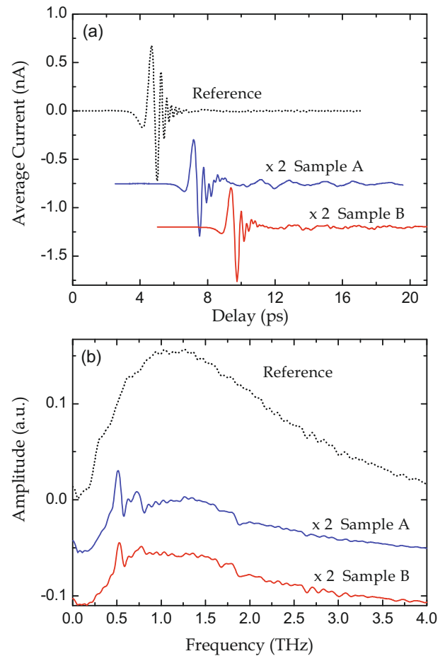
Fig. 5. (Color online) (a) Measured transmitted terahertz pulses and (b) the corresponding spectra through the reference and samples (multiplied by 2×). The curves in (a) and (b) are vertically displaced for clarity.
