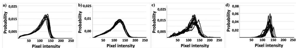
Fig. 7. PID graphs for peas for particular photo sizes: a) 1233 \times 1200 pixels; b) 733 \times 700 pixels; c) 233 \times 200 pixels; d) a single grain.
