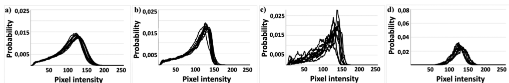
Fig. 8. PID graphs for pellets for particular photo sizes: a) 1233 \times 1200 pixels; b) 733 \times 700 pixels; c) 233 \times 200 pixels; d) a single grain.
