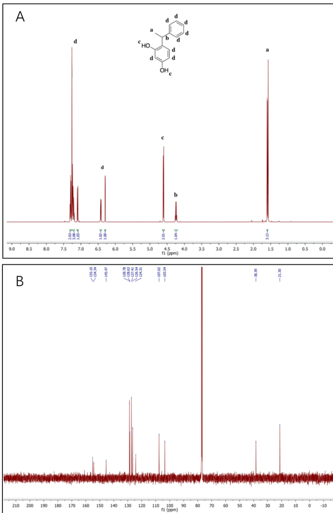
Figure 3. ^1\text{H} NMR (A) and ^{13}\text{C} NMR (B) spectrum of PR in d -chloroform.
