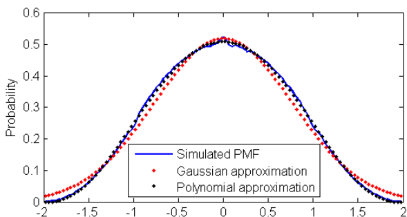
Fig. 15. PDF of modulation noise, \Delta_y , of a simulated MASH 1-1-1 modulator, showing the poor Gaussian fit (red) and the more appropriate polynomial fit used in the following examples (black).
