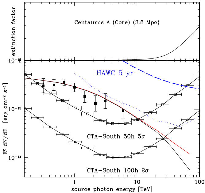
Fig. 7. Top panel: Photon–photon absorption correction ( \exp[\tau_{\gamma\gamma}] ) for the source Centaurus A at 3.8 Mpc, based on the EBL model by FR2017. Bottom panel: Observed (filled black squares) and model interpolated intrinsic spectrum (red line), and the absorption-corrected (black line) spectrum are reported. The two sensitivity limits for CTA are shown; see caption to Fig. 6
