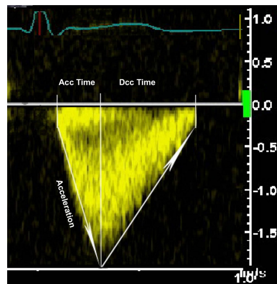
Fig. 2 Acceleration and deceleration times in pulmonary artery velocity profile. Acceleration time was the interval in \mu s from the onset of ejection to peak flow velocity. Deceleration time was measured from peak velocity to the end of ejection. Acc was the ratio of peak velocity in the pulmonary artery (PA) to the heart-rate-corrected acceleration time ( m/s^2 )
