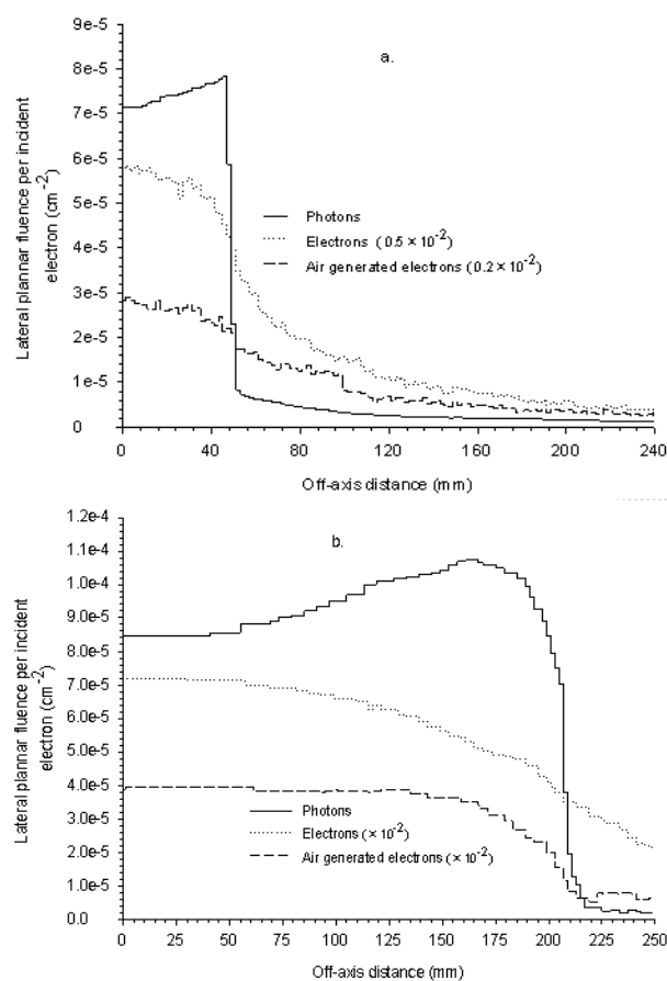
Figure 4. The planar fluence profiles of photons and electrons at the phantom surface for a. 10 \times 10 and b. 40 \times 40 \text{ cm}^2 field size at SSD =100 cm.
