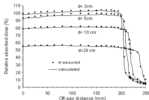
Figure 5. Comparison of the Monte Carlo dose profile calculations versus water phantom measurements for the 40 \times 40 \text{ cm}^2 field size at depths of 3, 5, 10 and 20 cm from up to down, respectively.
