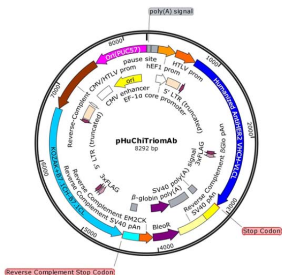
Figure 2. HuChiTriomAb expression vector. The no-cloning specific expression vector with a length less than 10 kbp and bidirectional expression potential for humanized antiHER2×human-B7.1: human-IgG1Fc tri-functional antibody with 94.3% human composition in silico was designed and then plotted using SnapGene software
