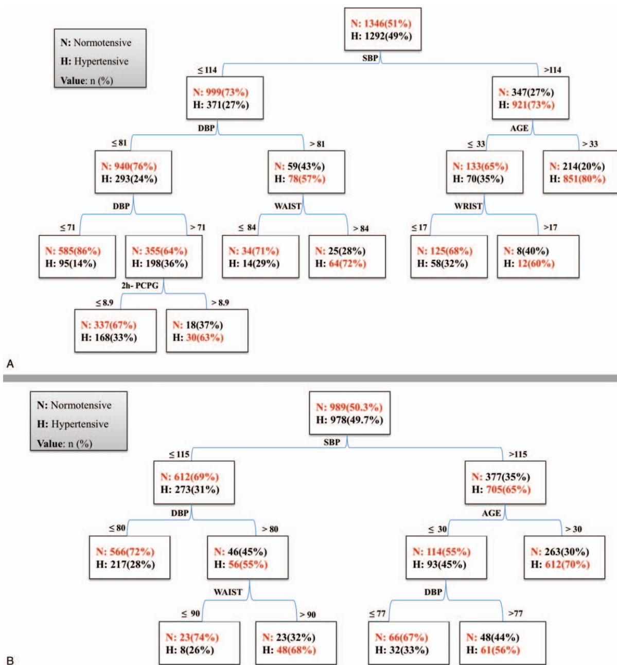
Figure 2. Decision tree models for prediction of hypertension derived from training dataset: (A) female population and (B) male population. Tehran Lipid and Glucose Study (1999–2012). 2h-PCPG=2-h postchallenge plasma glucose (mmol/L), DBP=diastolic blood pressure (mm Hg), SBP=systolic blood pressure (mm Hg), WAIST=waist circumference (cm).
