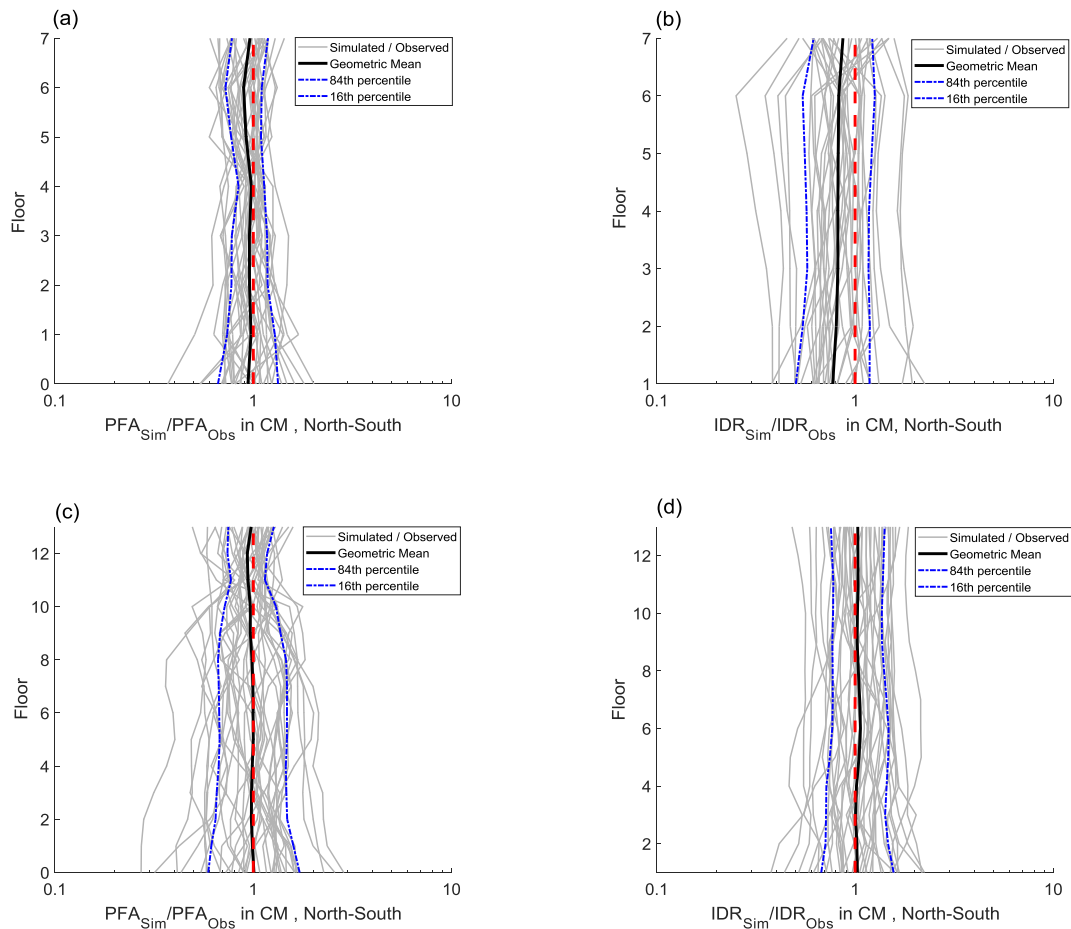
Figure 3: The ratios, geometric mean, and percentiles of simulated to observed responses (a) Building A peak floor acceleration (PFA); (b) Building A inter-storey drift (IDR); (c) Building B PFA; (d) Building B IDR.
