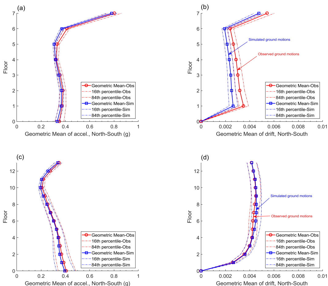
Figure 4: Geometric mean and percentiles of bootstrapped samples (a-b) Building A peak floor acceleration (PFA) and inter-storey drift ratio (IDR); (c-d) Building B PFA and IDR.
