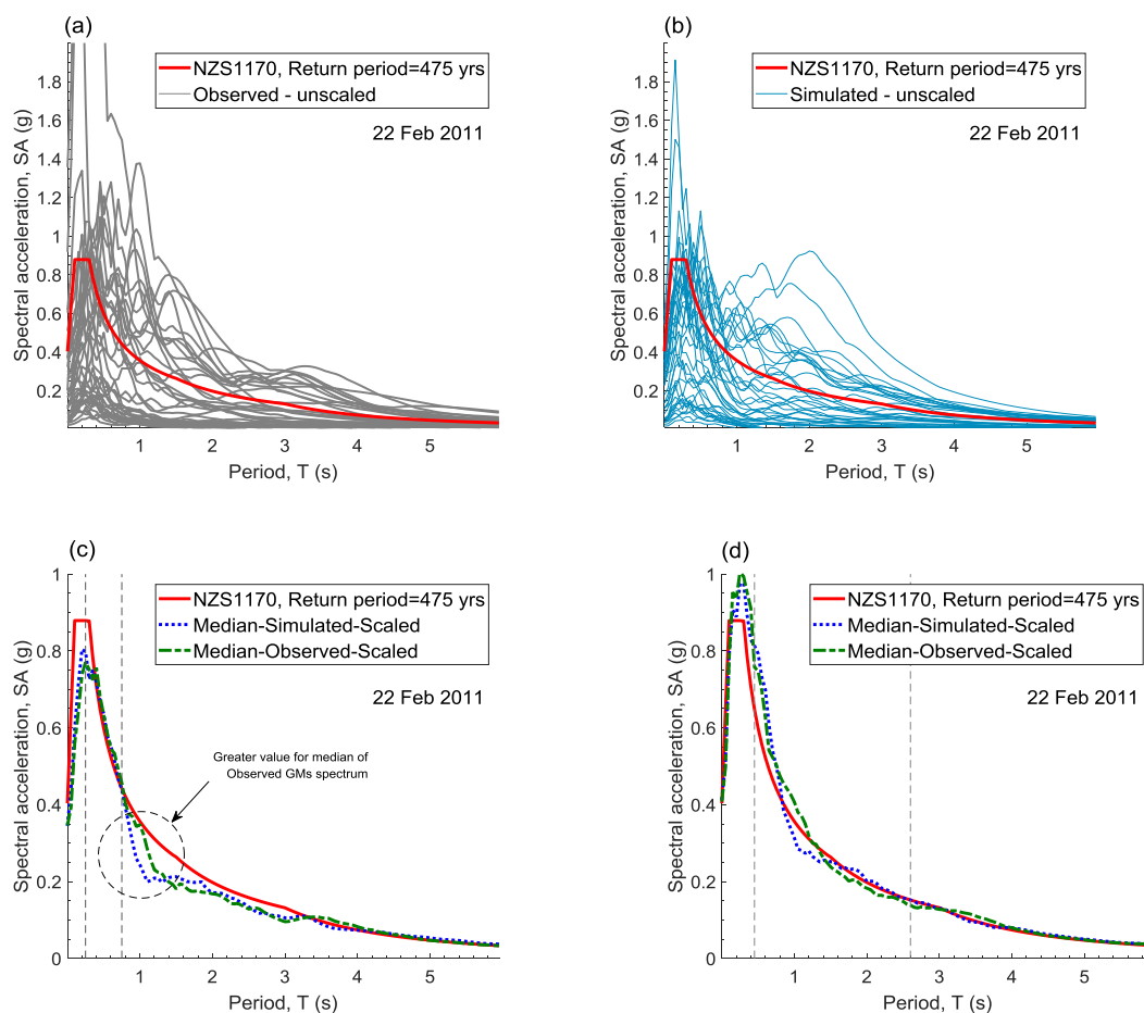
Figure 2: (a-b) Unscaled response spectra for the 40 observed and simulated GMs; (c-d) median of scaled response spectra for Building A and B.
