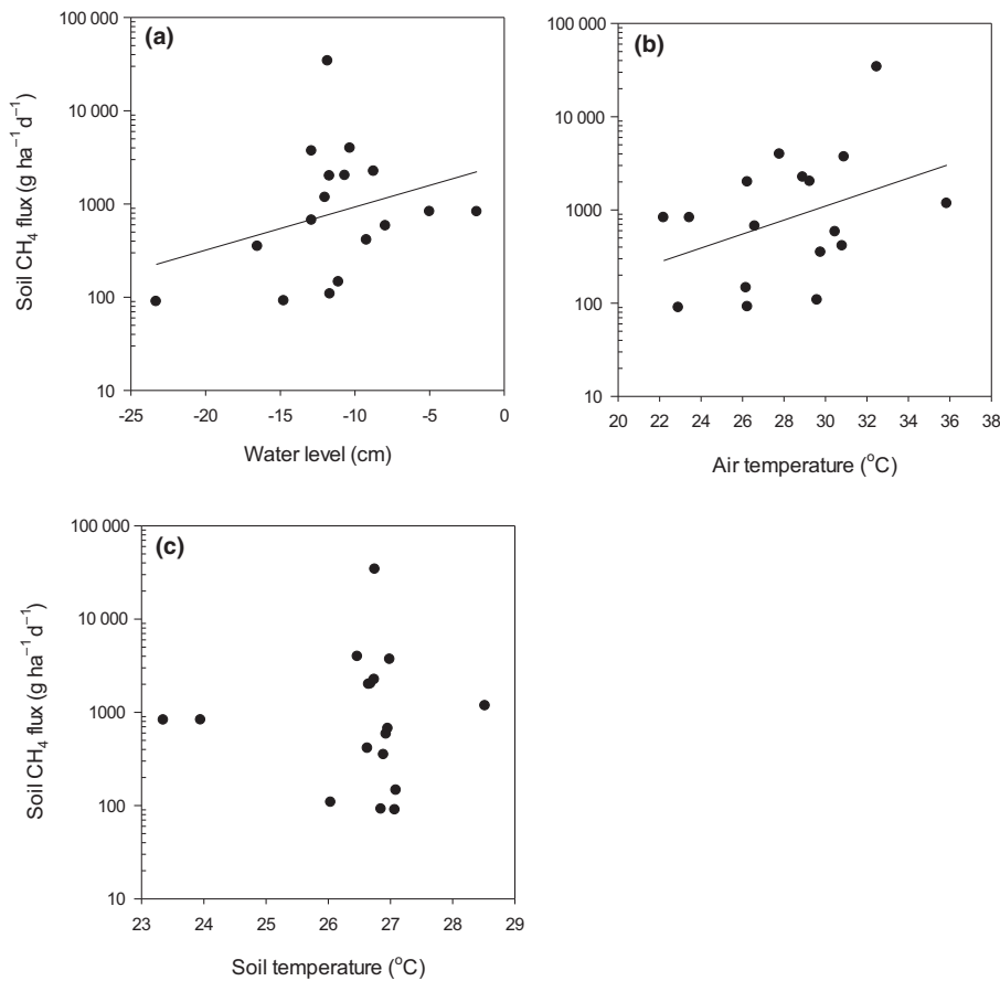
Fig. 6 Relationship between the mixed forest site \text{CH}_4 fluxes from the peat surface and (a) water levels (positive values indicate water levels above the peat surface), (b) air temperature and (c) soil temperature. Significant single linear regression lines are plotted; the models are reported in Table 3.
