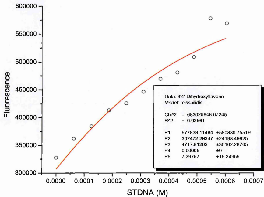
Figure 130: 3'4'-dihydroxyflavone – STDNA
