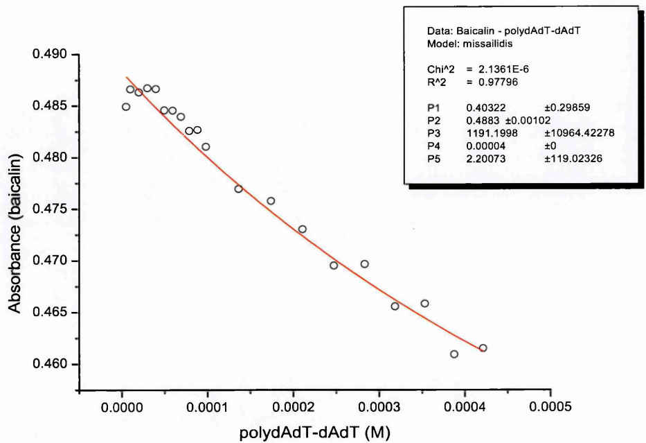
Figure 51: Baicalin – polydAdT-dAdT
