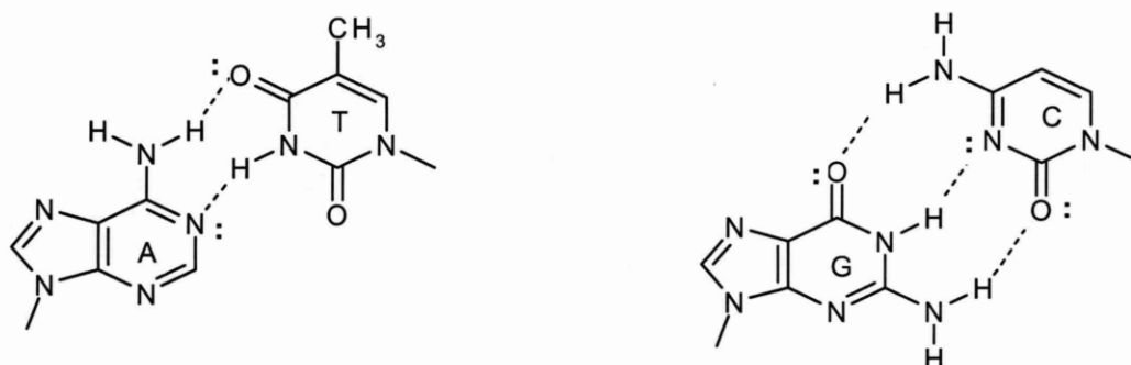
Figure 6: Hydrogen bonding (www.chembio.uoguelph.ca) between adenine - thymidine and guanine – cytosine.
