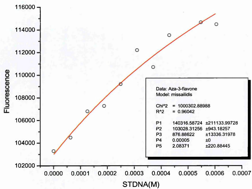
Figure 135: Aza-3-flavone - STDNA
