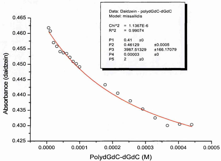
Figure 60: Daidzein – PolydGdC-dGdC
