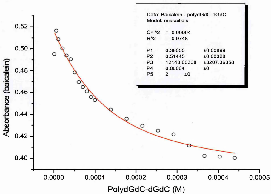
Figure 58: Baicalein – PolydGdC-dGdC
