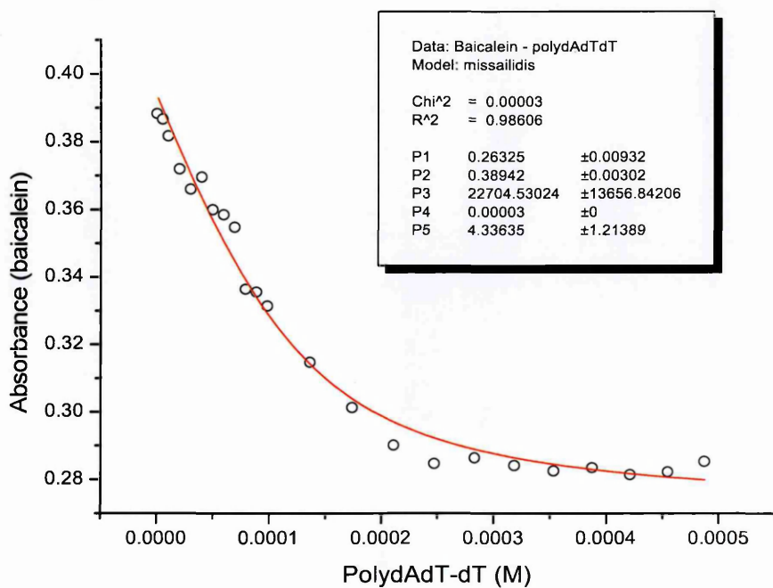
Figure 64: Baicalein – PolydAdT-dT
