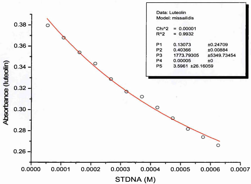
Figure 158: Luteolin – STDNA
