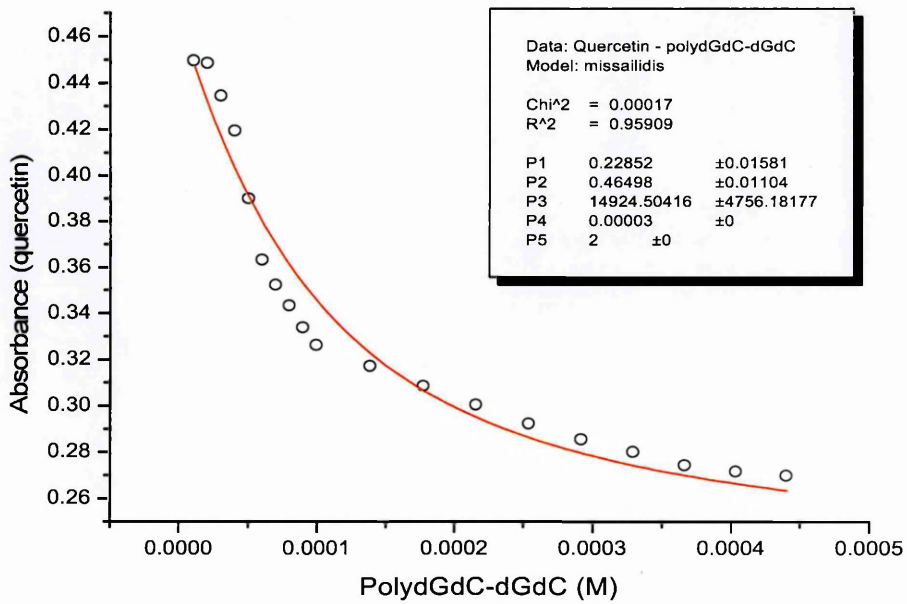
Figure 62: Quercetin – PolydGdC-dGdC
