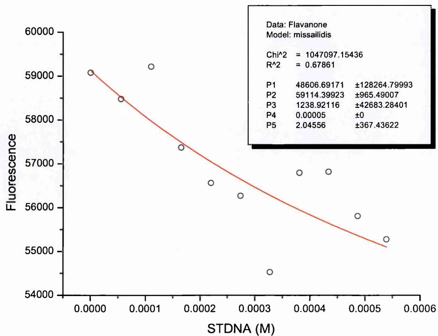
Figure 138: Flavanone - STDNA
