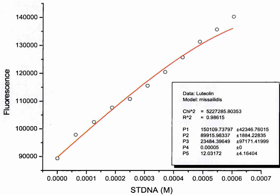
Figure 128: Luteolin – STDNA
