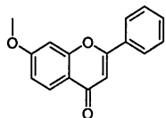
Compound 24
