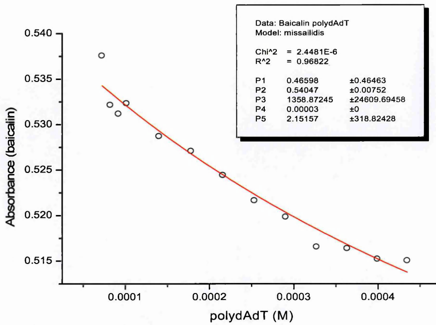
Figure 47: Baicalin - polydAdT
