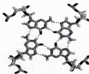
Figure 8: Guanine quartets ( www.il.mahidol.ac.th/.../quadruplex3.gif , 20/07/2006 )
