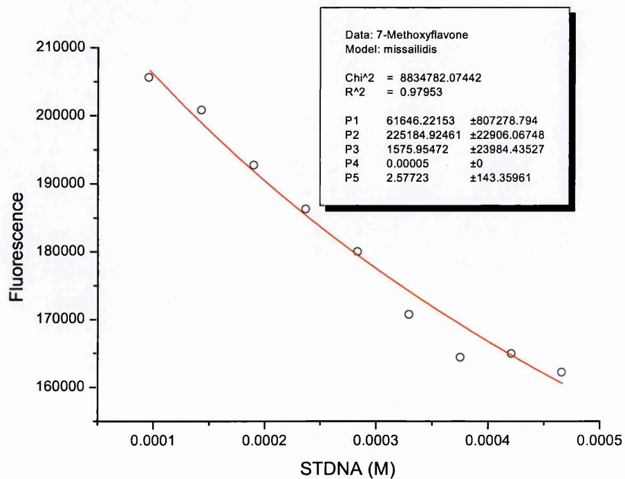
Figure 140: 7-methoxyflavone - STDNA
