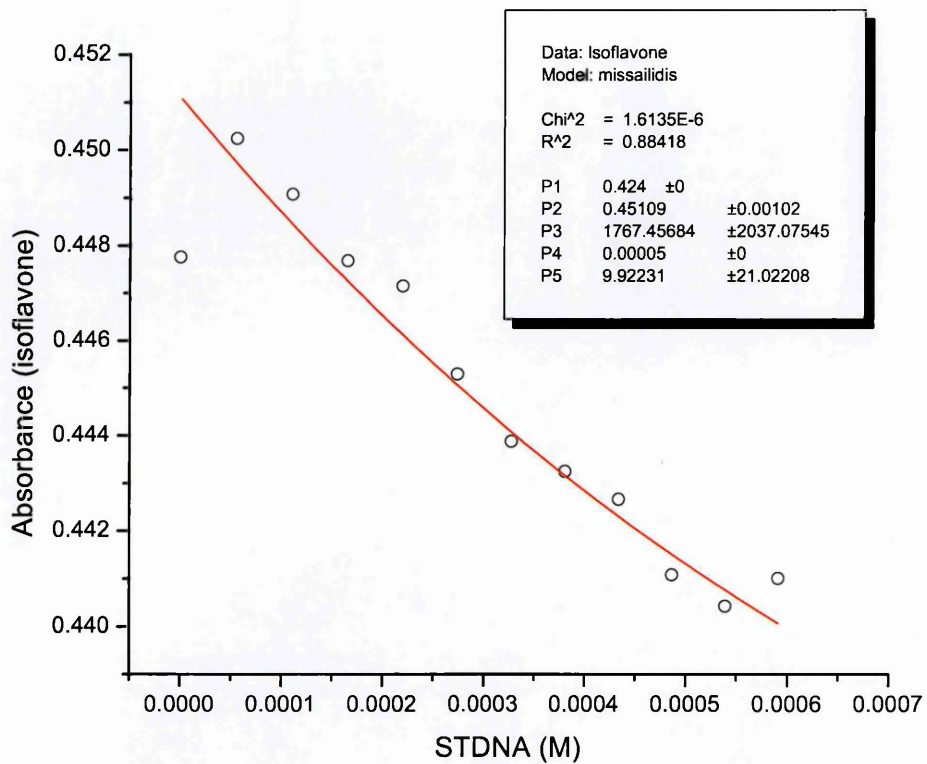
Figure 159: Isoflavone – STDNA
