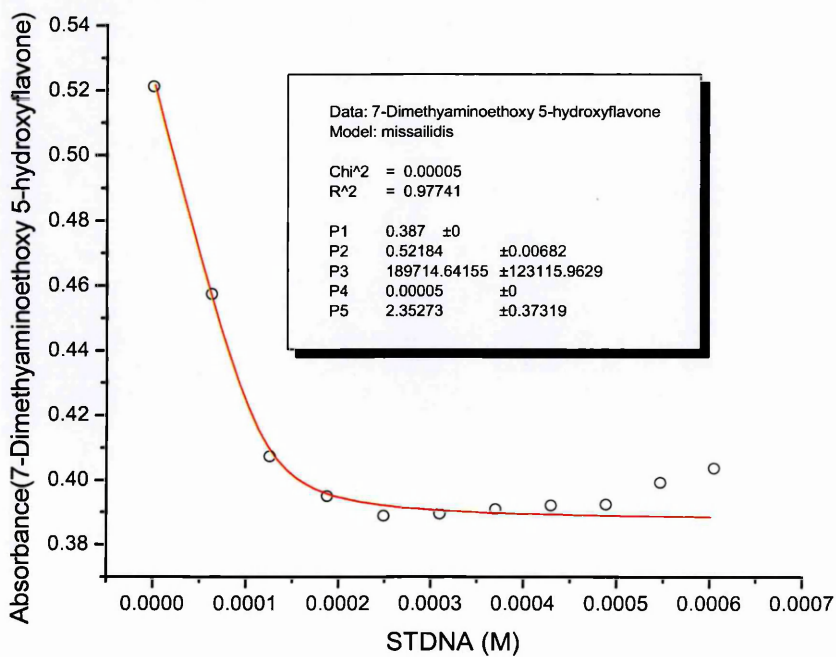
Figure 156: 7-dimethylaminoethoxy,5-hydroxyflavone – STDNA
