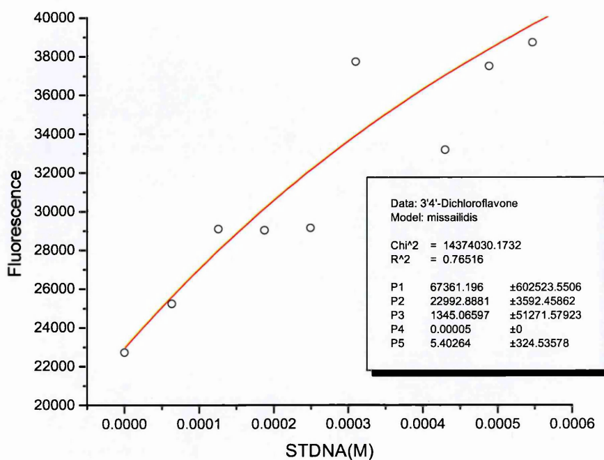
Figure 131: 3',4'-dichloroflavone – STDNA
