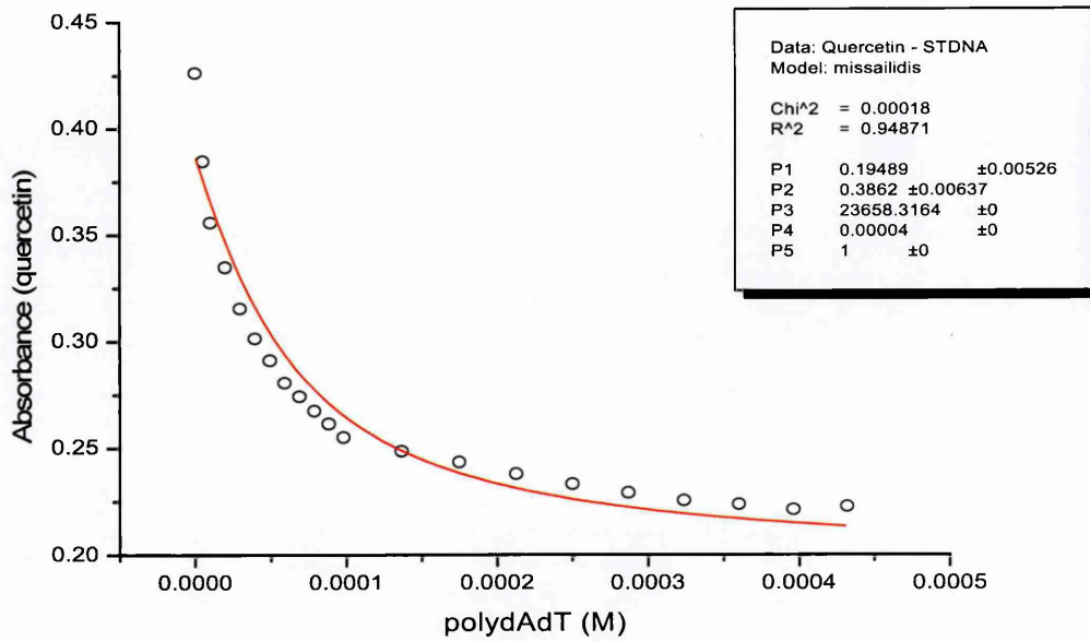
Figure 49: Quercetin - polydAdT
