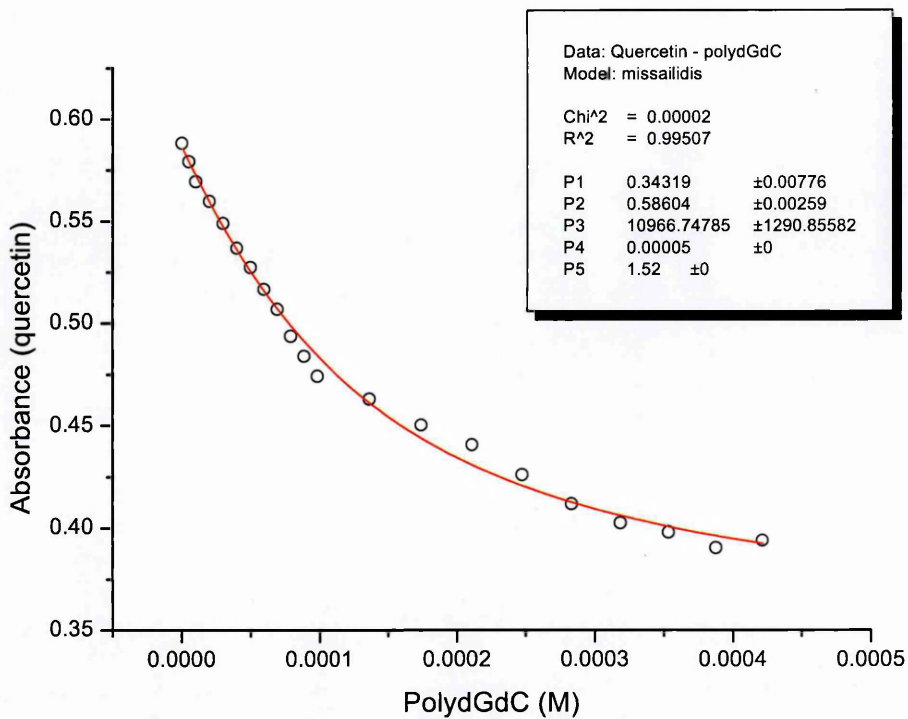
Figure 57: Quercetin – PolydGdC
