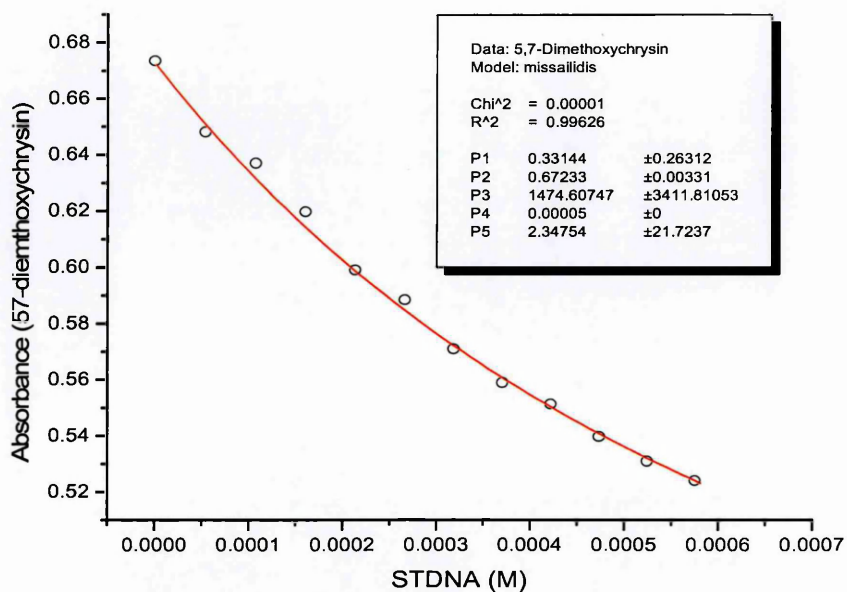
Figure 149: 5,7-dimethoxychrysin – STDNA
