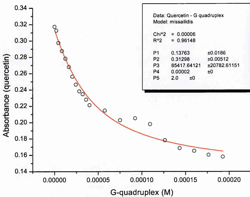
Figure 69: Quercetin – G-quadruplex
