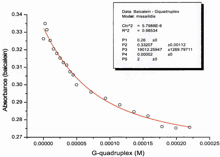
Figure 68: Baicalein – G-quadruplex
