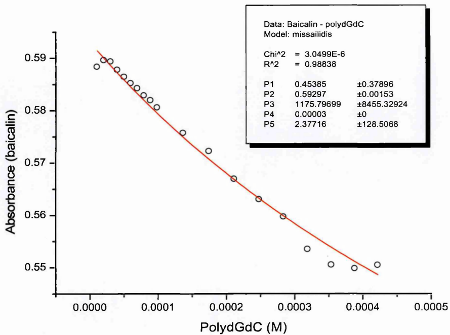
Figure 55: Baicalin - PolydGdC
