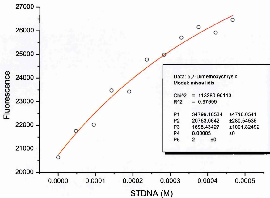
Figure 141: 5,7-dimethoxyflavone - STDNA
