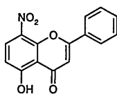
Compound 26
