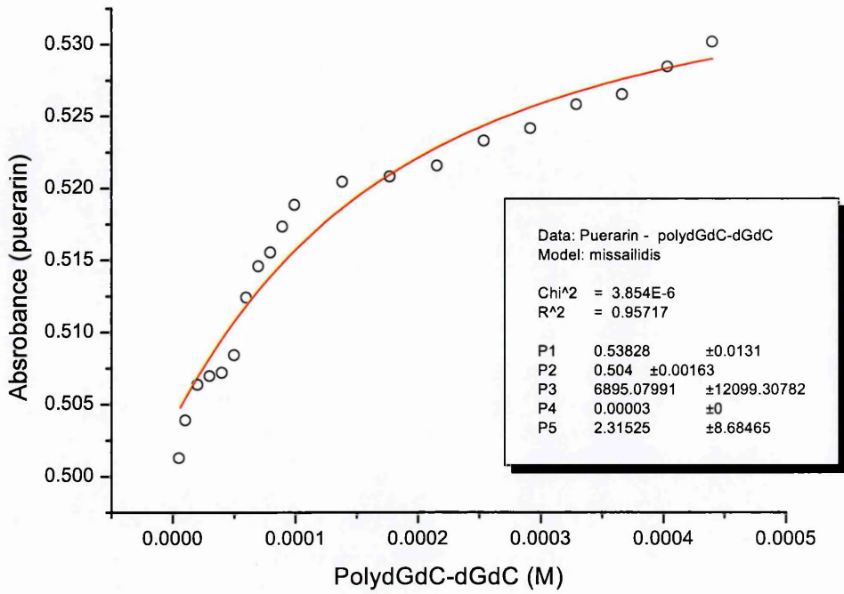
Figure 61: Puerarin – PolydGdC-dGdC
