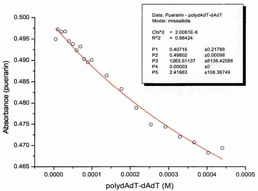
Figure 52: Puerarin – polydAdT-dAdT
