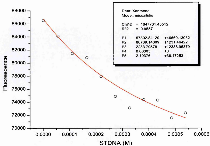
Figure 139: Xanthone – STDNA
