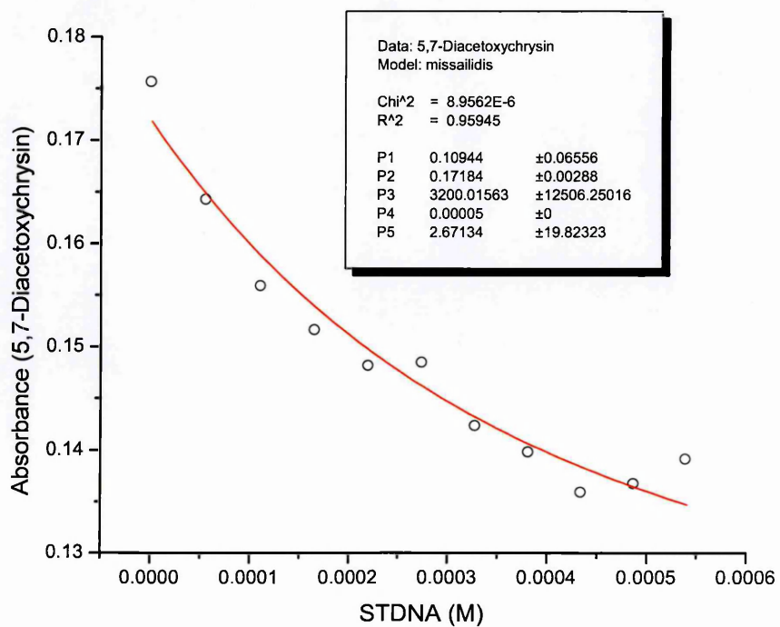
Figure 150: 5,7-diacetoxychrysin – STDNA
