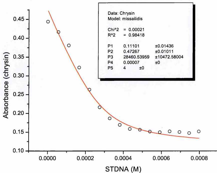
Figure 148: Chrysin - STDNA
