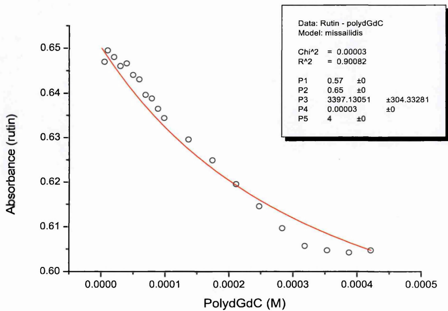
Figure 56: Rutin – PolydGdC
