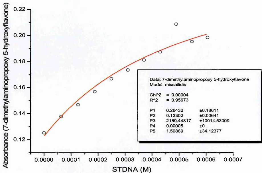
Figure 155: 7-dimethylaminopropoxy,5-hydroxyflavone – STDNA
