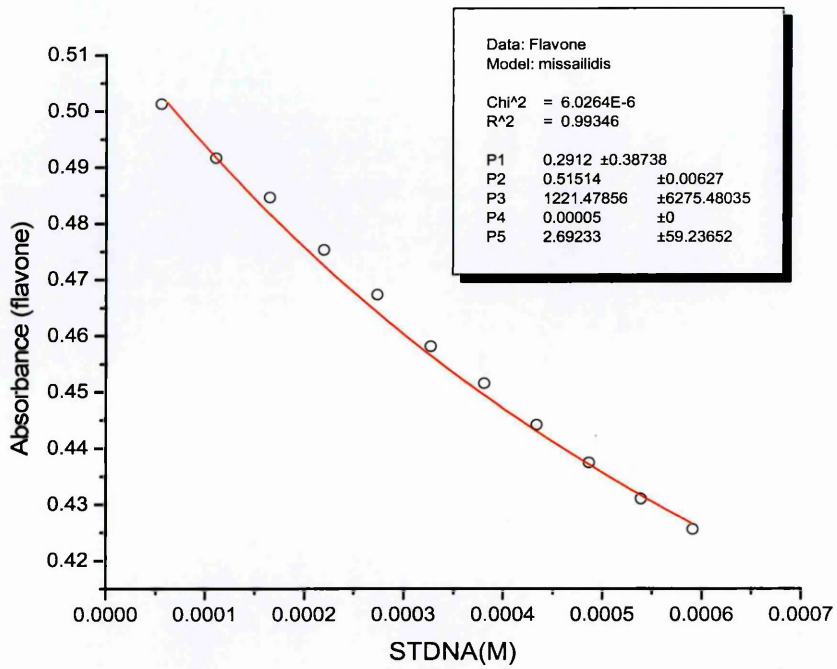
Figure 157: Flavone – STDNA
