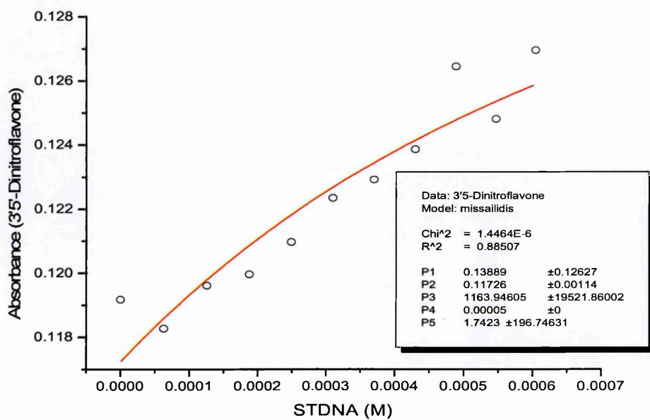
Figure 146: 3',5'-dinitroflavone – STDNA
