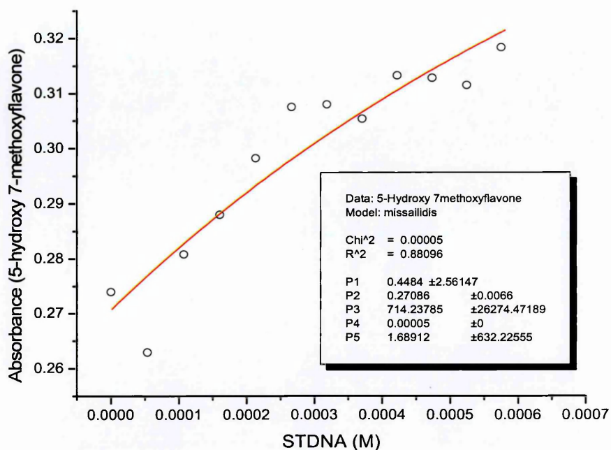
Figure 145: 5-hydroxy,7-methoxyflavone – STDNA
