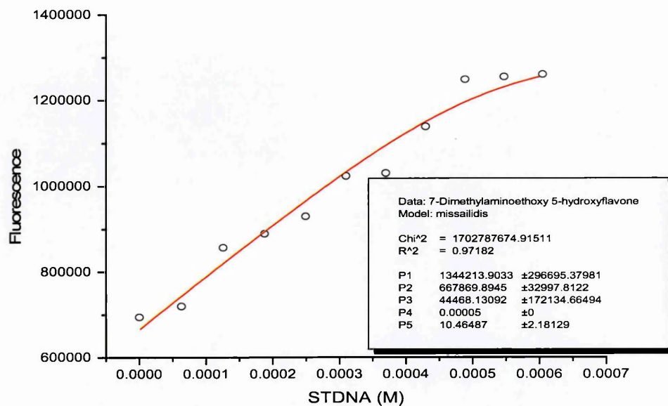
Figure 137: 7-dimethylaminoethoxy,5-hydroxyflavone – STDNA
