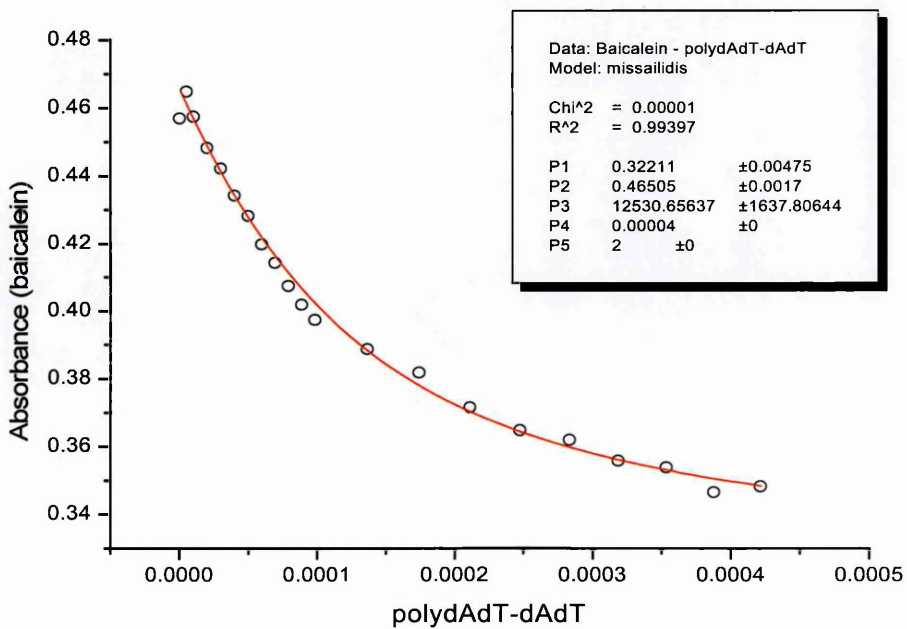
Figure 50: Baicalein polydAdT-dAdT
