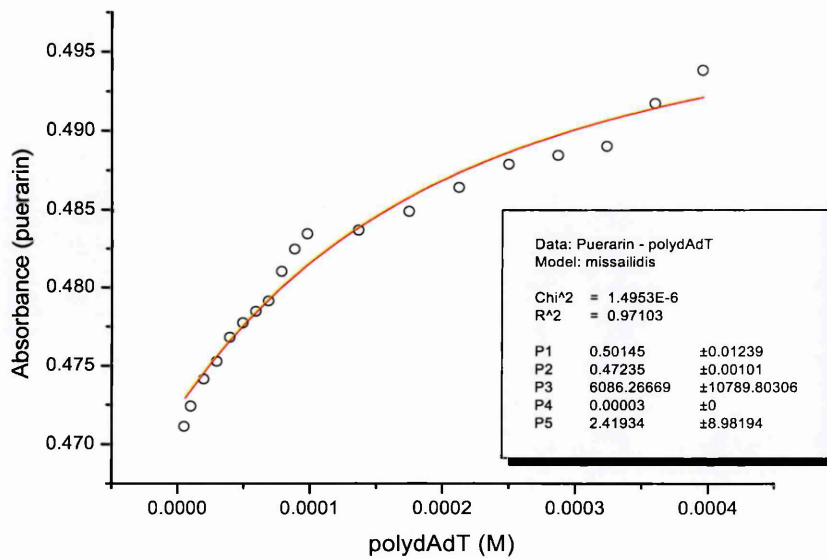
Figure 48: Puerarin - polydAdT
