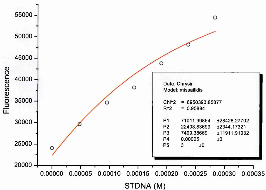
Figure 142: Chrysin – STDNA
