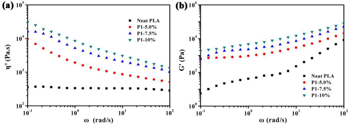
Fig. 7 Complex viscosity, \eta^* ( a ) and storage modulus, G' ( b ) plotted against frequency, \omega for the PLA and the PLA/lignin blends at the stain of 1 %.
