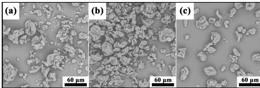
Fig. 3 SEM micrographs recorded on the PLA/lignin blends obtained; a) P1-5.0%, b) P1-7.5%, c) P1-10%.
