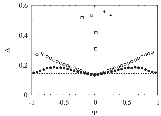
FIG. 2. Location of real score sheets on the \Psi - \Lambda plane. Solid diamonds and open boxes illustrate these features of the National Women's Handball Championship in the autumn and spring seasons of 2016-2017 in Hungary for the first and second classes. For n = 14 the \Psi dependence of the average values of the portion of hierarchical components is shown by solid and open circles for \rho = 0 and \rho = 0.5 . The dashed line shows the average value of \Lambda over the whole set of directed random graphs.
