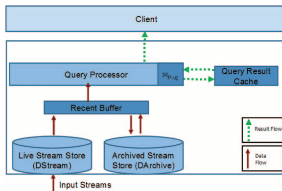
Figure 1: Architectural overview of the DeJaVu CEP system
