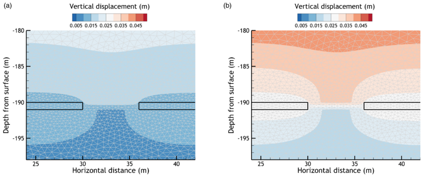
Fig. 6. Cross-section for one stall and two pillars (outlined in black) showing detail of modelled differential vertical displacement around pillar for a head change of (a) 20 m and (b) 40 m.
