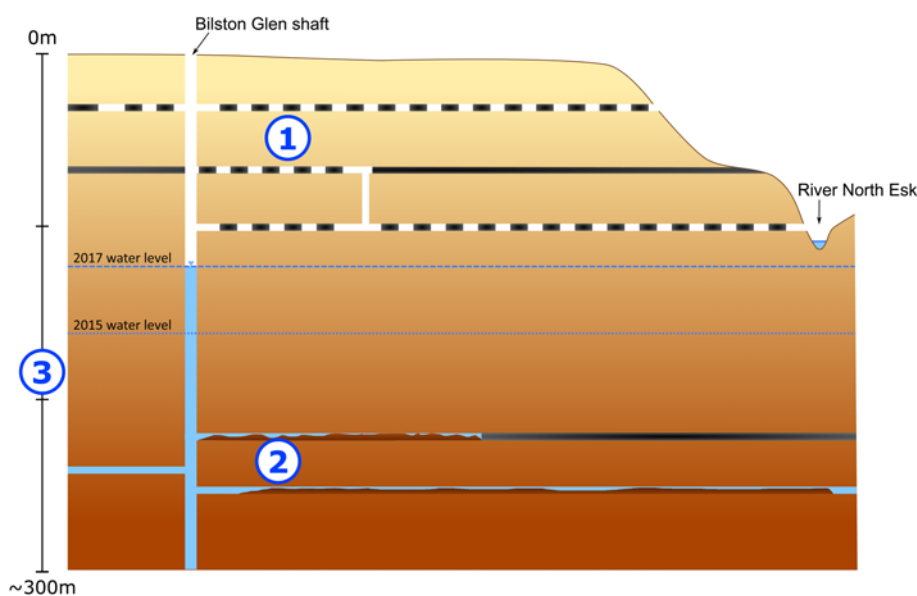
Fig. 1. Conceptual model set up using approximate surface elevations and mine water levels recorded in 2015 and 2017 from the Midlothian coalfield. (1) Pillar-and-stall mining (pillars shown in black, unsaturated pillars are shown in white), where columns of coal remaining to support the roof are commonly present in the top 100 m while (2) longwall mining, where the overburden is allowed to collapse into the workings known as ‘goaf’, are commonly deeper. The depth and dip of mine workings is schematic. (3) Approximate depth of model to ensure full saturation.
