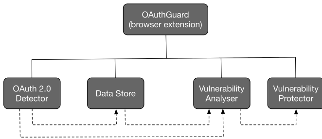
Figure 2: OAuthGuard Components
