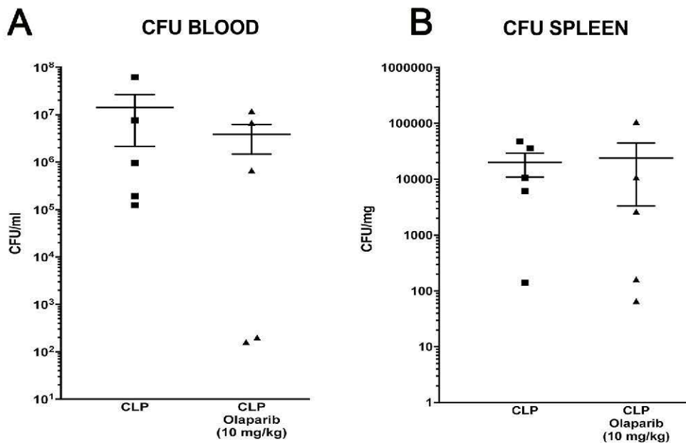
Fig. 18. Effect of olaparib on blood and spleen bacterial colony-forming unit (CFU) numbers in young female Balb/c mice subjected to CLP. (A): Blood CFUs (expressed as CFU/ml) and (B) spleen CFUs (expressed as CFU/mg) are shown in vehicle-treated mice subjected to CLP for 24 h ("CLP") and in mice subjected to CLP in the presence of 10 mg/kg olaparib ("CLP Olaparib 10 mg/kg"). Data are shown as mean \pm SEM of 10 animals for each group.
