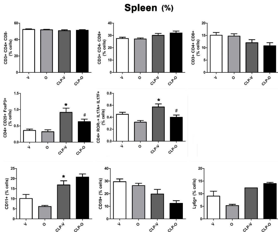
Fig. 13. Effect of olaparib on the percentages of various T-cell populations in the spleen of young male Balb/c mice subjected to CLP. Values are shown in sham mice (not subjected to CLP, but treated with vehicle for 24 h) ("V"), in sham mice (not subjected to CLP, but treated with 10 mg/kg olaparib for 24 h) ("O") in vehicle-treated mice subjected to CLP for 24 h ("CLP-V") and in mice subjected to CLP in the presence of 10 mg/kg olaparib ("CLP-O"). Data are shown as mean \pm SEM of 10 animals for each group; *p < 0.05 shows a significant change in the respective cell population in response to CLP, compared to the sham group; #p < 0.05 shows significant effect of olaparib under non-CLP conditions (compared to vehicle-treated sham mice) or in CLP mice (compared to vehicle-treated CLP mice).
