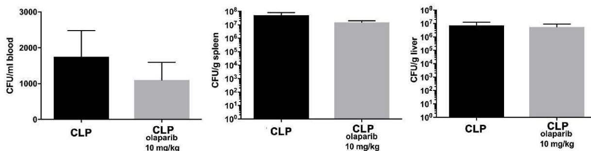
Fig. 10. Effect of olaparib on blood, spleen and liver bacterial colony-forming unit (CFU) numbers in young male Balb/c mice subjected to E. coli bacteria in vivo . Blood (expressed as CFU/ml), spleen and liver CFUs (expressed as CFU/g) are shown in vehicle-treated mice inoculated with E. coli for 24 h ("CLP") and in mice subjected to CLP in the presence of 10 mg/kg olaparib. Data are shown as mean \pm SEM of 6 animals for each group.
