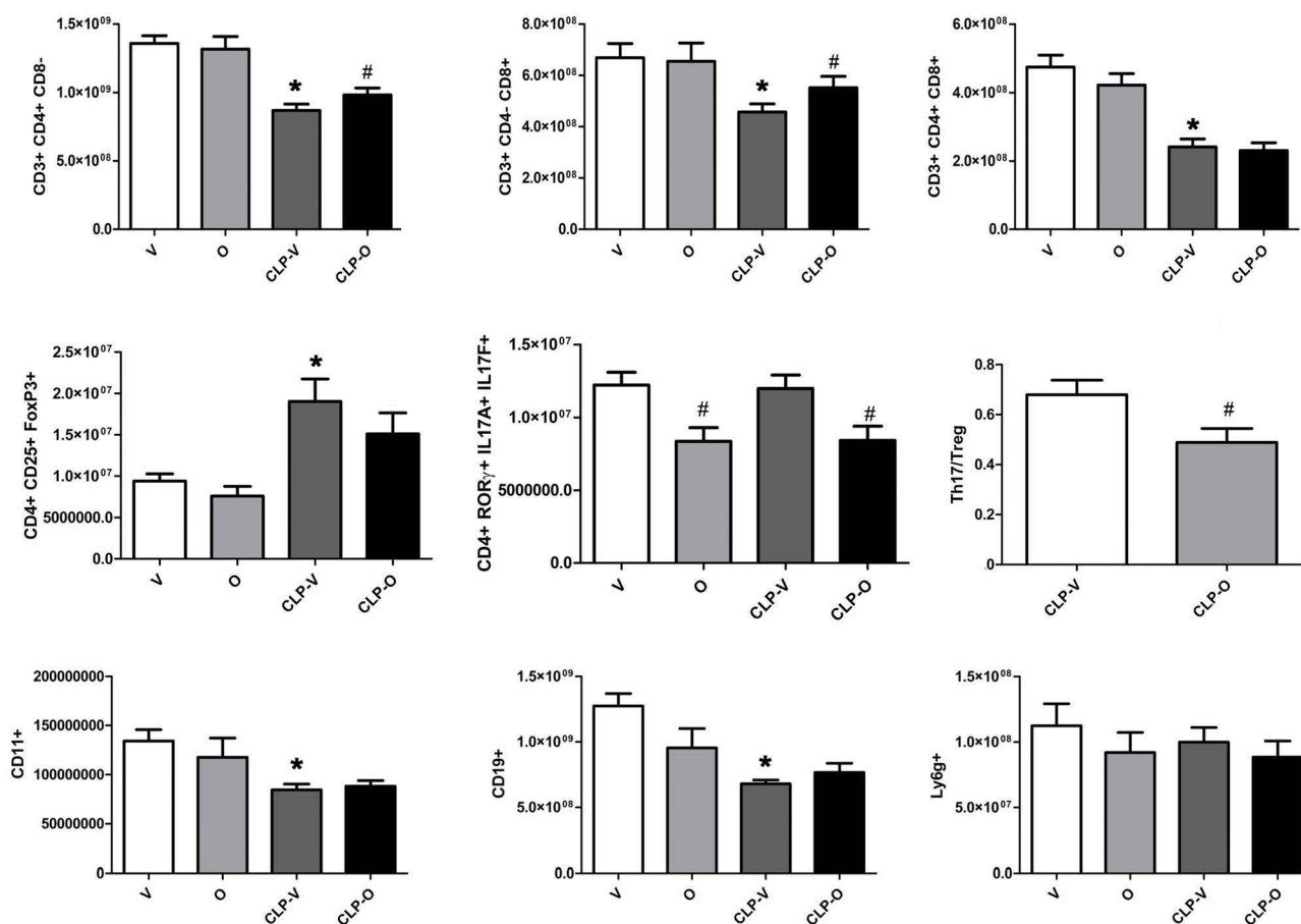
Fig. 12. Effect of olaparib on the numbers of various T-cell populations in the spleen of young male Balb/c mice subjected to CLP. Values are shown in sham mice (not subjected to CLP, but treated with vehicle for 24 h) ("V"), in sham mice (not subjected to CLP, but treated with 10 mg/kg olaparib for 24 h) ("O") in vehicle-treated mice subjected to CLP for 24 h ("CLP-V") and in mice subjected to CLP in the presence of 10 mg/kg olaparib ("CLP-O"). Data are shown as mean \pm SEM of 10 animals for each group; *p < 0.05 shows a significant change in the respective cell population in comparison to the sham group; #p < 0.05 shows significant effect of olaparib under non-CLP conditions (compared to vehicle-treated sham mice) or in CLP mice (compared to vehicle-treated CLP mice).
