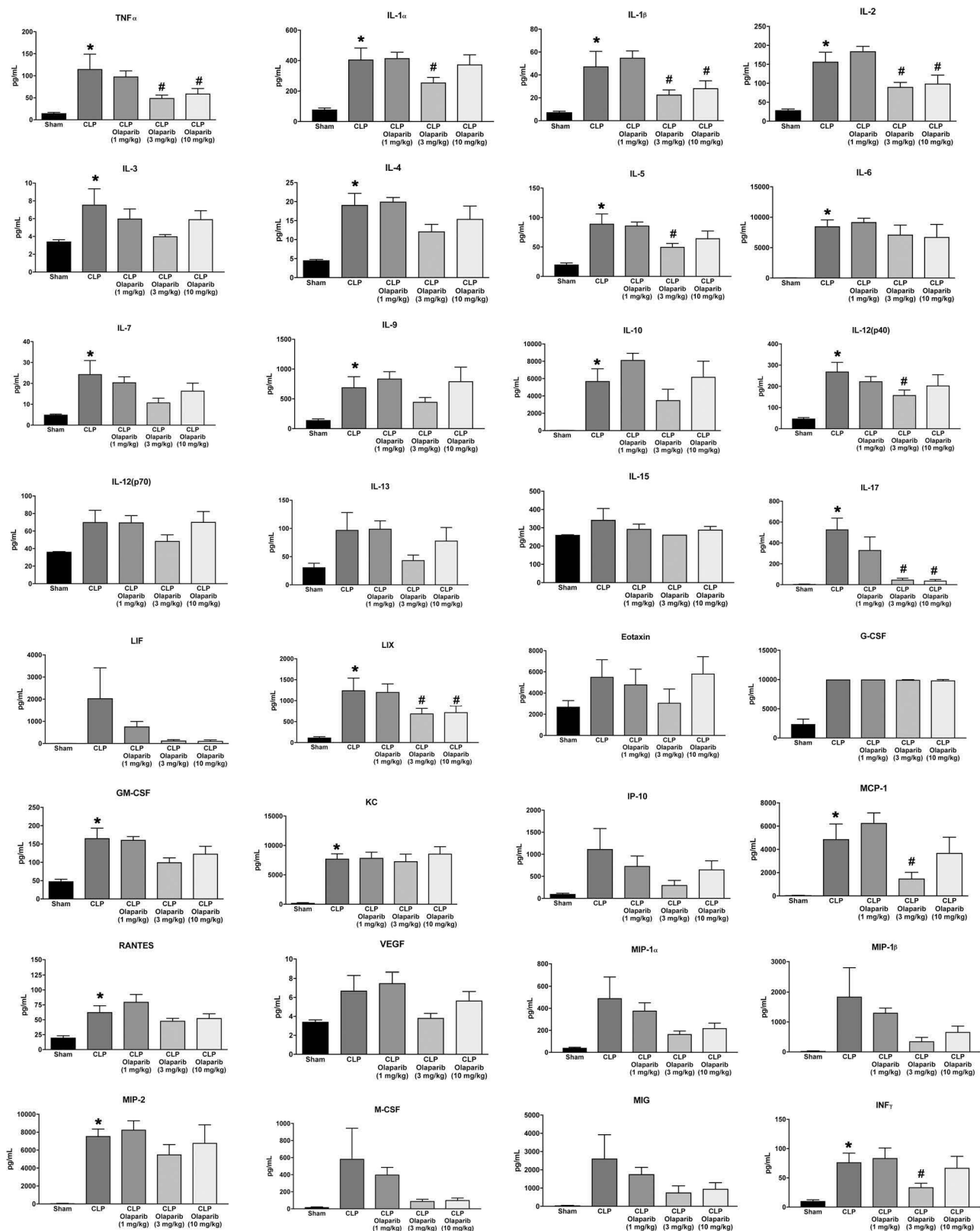
Fig. 11. Effect of olaparib on the levels of various circulating mediators (cytokines, chemokines, growth factors) in young male Balb/c mice subjected to CLP. Values are shown in sham mice (not subjected to CLP) ("Sham"), in vehicle-treated mice subjected to CLP for 24 h ("CLP") and in mice subjected to CLP in the presence of various doses of olaparib ("CLP Olaparib 1 mg/kg", "CLP Olaparib 3 mg/kg" and "CLP Olaparib 10 mg/kg"). Data are shown as mean \pm SEM of 10 animals for each group; * p < 0.05 shows significant increase in the respective parameter in response to CLP, compared to the sham group; # p < 0.05 shows significant protective effect of olaparib in CLP mice compared to vehicle-treated CLP mice.
