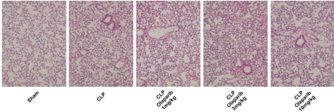
Fig. 3. Effect of olaparib on histological alterations injury in the lungs of young male Balb/c mice subjected to CLP. Representative histological pictures are shown in sham mice (not subjected to CLP) ("Sham"), in vehicle-treated mice subjected to CLP for 24 h ("CLP") and in mice subjected to CLP in the presence of various doses of olaparib ("CLP Olaparib 1 mg/kg", "CLP Olaparib 3 mg/kg" and "CLP Olaparib 10 mg/kg"). Pictures are selected from n = 5 animals for each group.
