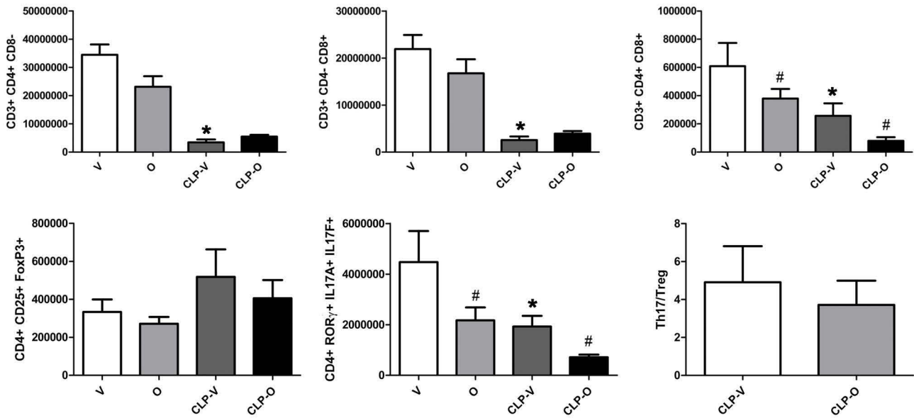
Fig. 14. Effect of olaparib on the numbers of various T-cell populations in the blood of young male Balb/c mice subjected to CLP. Values are shown in sham mice (not subjected to CLP, but treated with vehicle for 24 h) ("V"), in sham mice (not subjected to CLP, but treated with 10 mg/kg olaparib for 24 h) ("O") in vehicle-treated mice subjected to CLP for 24 h ("CLP-V") and in mice subjected to CLP in the presence of 10 mg/kg olaparib ("CLP-O"). Data are shown as mean \pm SEM of 10 animals for each group; * p < 0.05 shows a significant change in the respective cell population in response to CLP, compared to the sham group; # p < 0.05 shows significant effect of olaparib under non-CLP conditions (compared to vehicle-treated sham mice) or in CLP mice (compared to vehicle-treated CLP mice).
