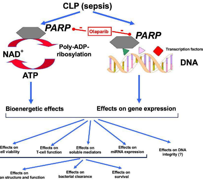
Fig. 31. Effects of olaparib in septic shock: a working hypothesis. via inhibition of the catalytic activity of PARP, olaparib exerts cellular bioenergetic effects as well as pluripotent modulation of gene transcription. These effects lead to changes in the circulating and tissue-resident immune cell distribution, improve bacterial elimination, protect against multiorgan injury and eventually culminate in improved survival rate. These effects are dependent on gender and age of the animals. See the Discussion section for further context and explanation.
