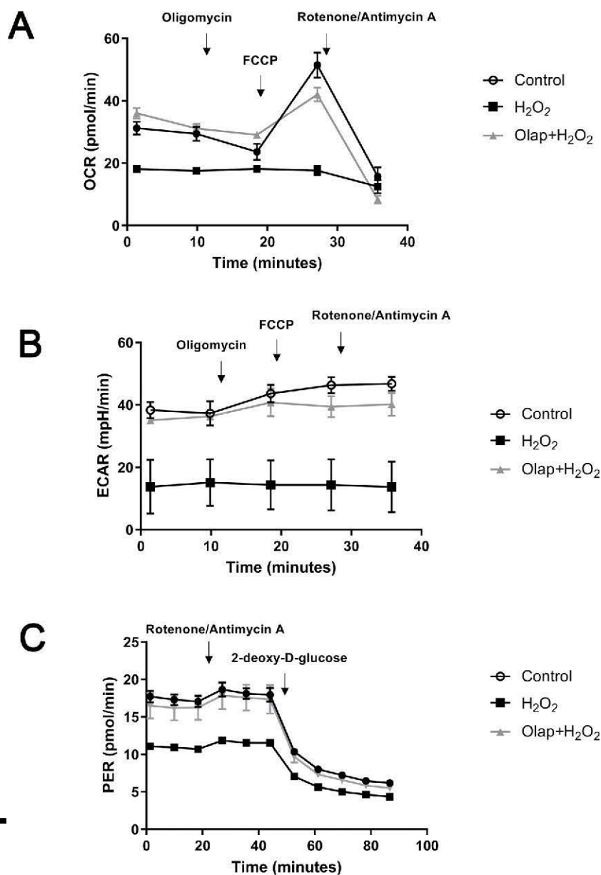
Fig. 26. Effect of olaparib on bioenergetic parameters in U937 cells subjected to H 2 O 2 -induced oxidative stress in vitro . (A): Representative oxygen consumption rate (OCR) profiles in control cells, in H 2 O 2 (300 μM) treated cells at 1 h, and in H 2 O 2 (300 μM) treated cells at 1 h in the presence of pretreatment with 10 μM olaparib. Arrows indicate the addition of specific mitochondria stressors. Results are indicated as mean ± SEM of n = 3 per condition. (B): Representative extracellular acidification rate (ECAR) profiles in control cells, in H 2 O 2 (300 μM) treated cells at 1 h, and in H 2 O 2 (300 μM) treated cells at 1 h in the presence of pretreatment with 10 μM olaparib. Arrows indicate the addition of specific mitochondria stressors into the media. Results are indicated as mean ± SEM of n = 3 per condition. (C): Representative proton efflux rate (PER) profiles in control cells, in H 2 O 2 (300 μM) treated cells at 1 h, and in H 2 O 2 (300 μM) treated cells at 1 h in the presence of pretreatment with 10 μM olaparib. Arrows indicate the addition of specific mitochondria stressors into the media. Results are indicated as mean ± SEM of n = 3 per condition.
