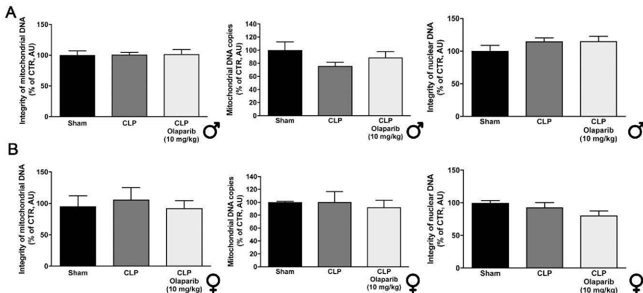
Fig. 23. Effect of olaparib on liver mitochondrial DNA integrity, mitochondrial DNA copy number and nuclear DNA integrity in aged male and female Balb/c mice subjected to CLP. (A): mitochondrial DNA integrity, mitochondrial DNA copy number and nuclear DNA integrity values (expressed as % of control) in aged male mice; (B): mitochondrial DNA integrity, mitochondrial DNA copy number and nuclear DNA integrity values (expressed as % of control) in aged female mice. Data are shown in sham mice (not subjected to CLP) ("Sham"), in vehicle-treated mice subjected to CLP for 24 h ("CLP") and in mice subjected to CLP in the presence of 10 mg/kg olaparib ("CLP Olaparib 10 mg/kg"). Data are shown as mean \pm SEM of 10 animals for each group.
