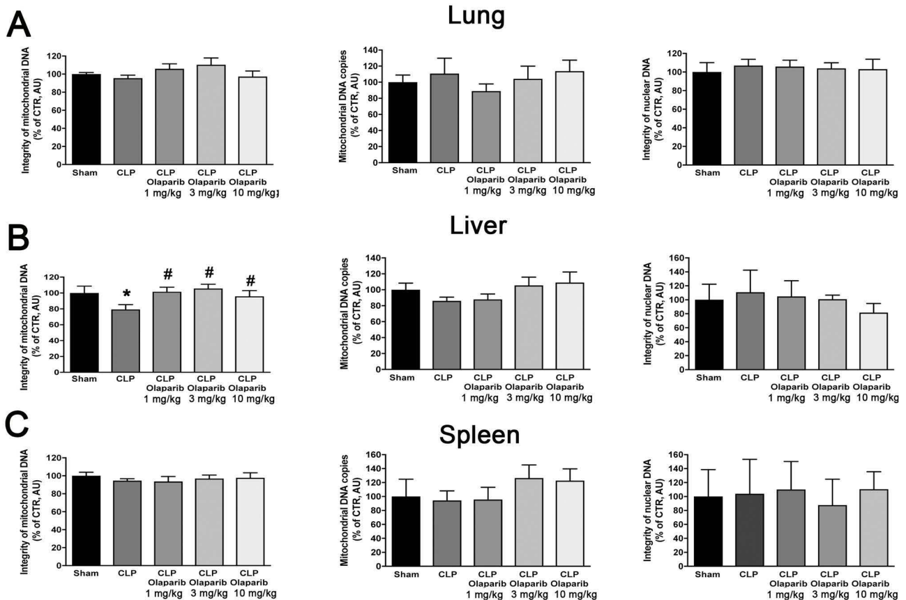
Fig. 7. Effect of olaparib on lung, liver and spleen mitochondrial DNA integrity, mitochondrial DNA copy number and nuclear DNA integrity in young male Balb/c mice subjected to CLP. (A): Lung mitochondrial DNA integrity, mitochondrial DNA copy number and nuclear DNA integrity values (expressed as % of control); (B): liver mitochondrial DNA integrity, mitochondrial DNA copy number and nuclear DNA integrity values (expressed as % of control); (C) spleen mitochondrial DNA integrity, mitochondrial DNA copy number and nuclear DNA integrity values (expressed as % of control) are shown in sham mice (not subjected to CLP) ("Sham"), in vehicle-treated mice subjected to CLP for 24 h ("CLP") and in mice subjected to CLP in the presence of various doses of olaparib ("CLP Olaparib 1 mg/kg", CLP Olaparib 3 mg/kg" and "CLP Olaparib 10 mg/kg"). Data are shown as mean \pm SEM of 10 animals for each group; * p < 0.05 shows significant change in a respective parameter in response to CLP, compared to the sham group; # p < 0.05 shows significant effect of olaparib on a given parameter in CLP mice compared to vehicle-treated CLP mice.
