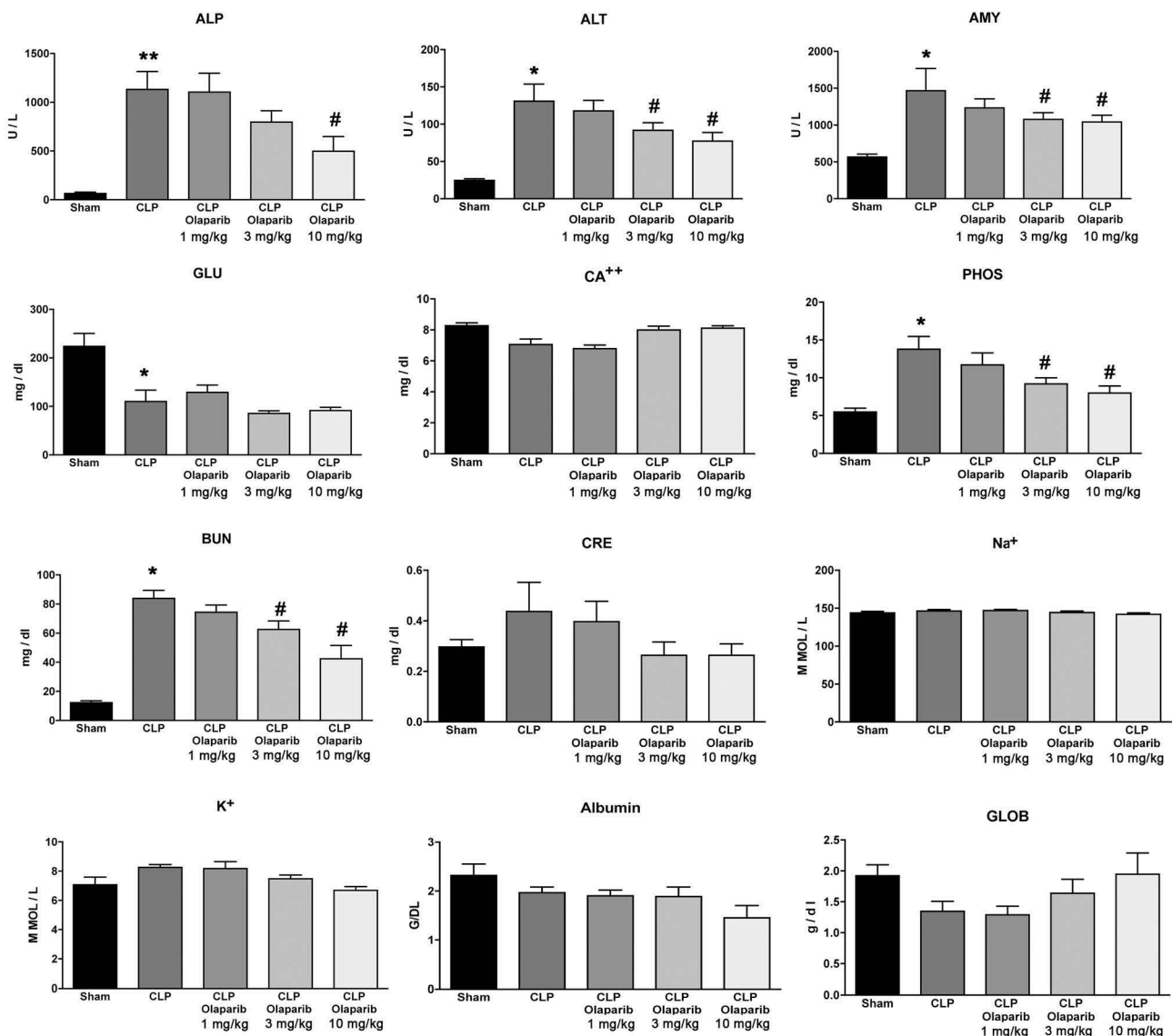
Fig. 2. Effect of olaparib on selected parameters of organ injury in young male Balb/c mice subjected to CLP. Various physiological and organ injury marker levels: alkaline phosphatase (ALP), alanine aminotransferase (ALT), amylase (AMY), plasma glucose (GLU), plasma calcium (CA ++ ), plasma phosphate (PHOS), plasma blood urea nitrogen (BUN), plasma creatinine (CRE), plasma sodium (Na + ), plasma potassium (K + ), plasma albumin (ALB) and plasma globulin (GLOB) measured by Vetscan analysis, are shown in sham mice (not subjected to CLP) ("Sham"), in vehicle-treated mice subjected to CLP for 24 h ("CLP") and in mice subjected to CLP in the presence of various doses of olaparib ("CLP Olaparib 1 mg/kg", "CLP Olaparib 3 mg/kg" and "CLP Olaparib 10 mg/kg"). Data are shown as mean ± SEM of 10 animals for each group; *p < 0.05 shows significant increase in the respective parameter in response to CLP, compared to the sham group; #p < 0.05 shows significant protective effect of olaparib in CLP mice compared to vehicle-treated CLP mice.
