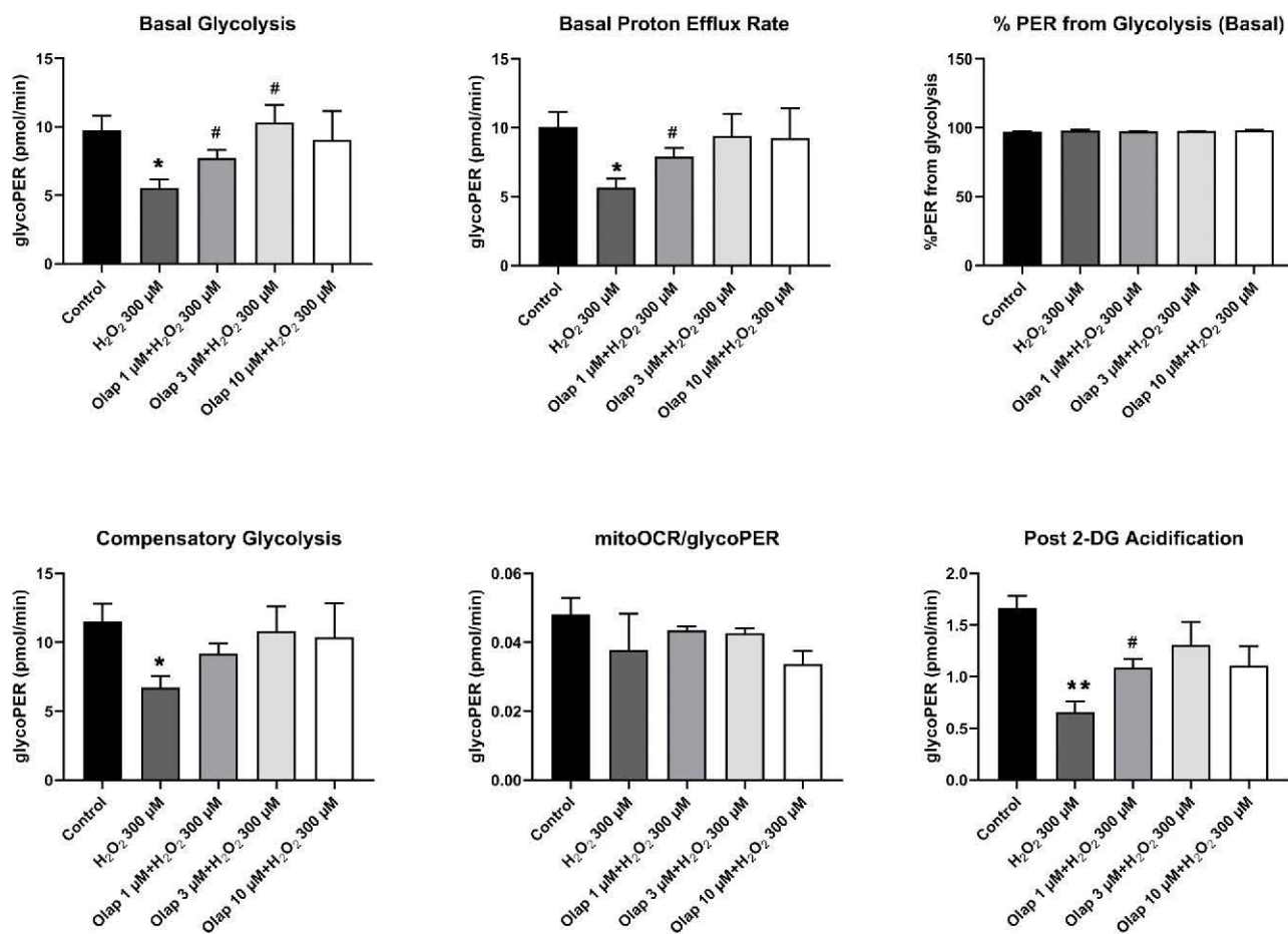
Fig. 28. Effect of olaparib on glycolysis-related bioenergetic parameters in U937 cells subjected to H 2 O 2 -induced oxidative stress in vitro . Results are shown in control cells, in H 2 O 2 (300 μM) treated cells at 1 h, and in H 2 O 2 (300 μM) treated cells at 1 h in the presence of pretreatment with 1, 3 or 10 μM olaparib. Results are indicated as mean ± SEM of n = 3 per condition. *p < 0.05 shows a significant change in response to H 2 O 2 , compared to control cells; #p < 0.05 shows significant protective effect of olaparib in H 2 O 2 challenged cells compared to vehicle-treated H 2 O 2 challenged cells.
