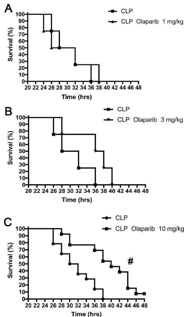
Fig. 6. Effect of olaparib on the survival rate of young male Balb/c mice subjected to CLP. Survival rates are shown in mice subjected to CLP in the presence of various doses of olaparib ("CLP Olaparib 1 mg/kg", CLP Olaparib 3 mg/kg" and "CLP Olaparib 10 mg/kg"). Data are shown as mean \pm SEM of 10–12 animals for each group; # p < 0.05 shows significant protective effect of olaparib in CLP mice compared to vehicle-treated CLP mice.
