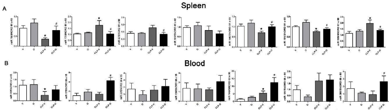
Fig. 16. Effect of olaparib on spleen and blood T-cell miRNA levels in young male Balb/c mice subjected to CLP. Values are shown in sham mice (not subjected to CLP, but treated with vehicle for 24 h) ("V"), in sham mice (not subjected to CLP, but treated with 10 mg/kg olaparib for 24 h) ("O") in vehicle-treated mice subjected to CLP for 24 h ("CLP-V") and in mice subjected to CLP in the presence of 10 mg/kg olaparib ("CLP-O"). Data are shown as mean \pm SEM of 10 animals for each group; * p < 0.05 shows a significant change in the respective miRNA level in response to CLP, compared to the sham group; # p < 0.05 shows significant effect of olaparib under non-CLP conditions (compared to vehicle-treated sham mice) or in CLP mice (compared to vehicle-treated CLP mice).
