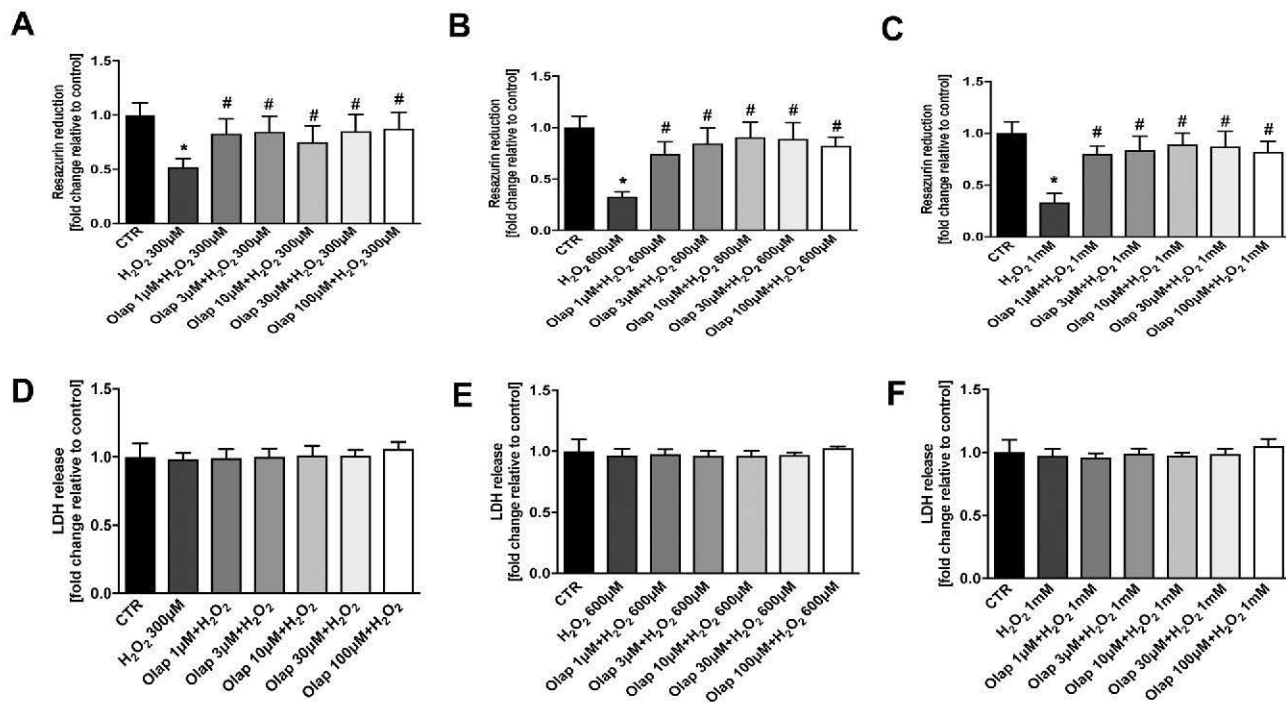
Fig. 25. Effect of olaparib on cellular viability in U937 cells subjected to H 2 O 2 -induced oxidative stress in vitro . (A): Effect of olaparib on cellular resazurin reduction in control cells (without oxidative stress challenge) and in cells subjected to oxidative (H 2 O 2 ) in the presence of various concentrations of olaparib. Cells were treated with olaparib (1, 3, 10, 30 or 100 μM), followed immediately by 300 μM H 2 O 2 for 1 h. Data are shown as mean ± SEM of n = 3 determinations. *p < 0.05 shows significant decrease in resazurin conversion in response to H 2 O 2 , compared to control cells; #p < 0.05 shows significant protective effect of olaparib in H 2 O 2 challenged cells compared to vehicle-treated H 2 O 2 challenged cells. (B): Effect of olaparib on LDH content (a marker of cell necrosis) in the supernatant of control cells (without oxidative stress challenge) and in cells subjected to oxidative (H 2 O 2 ) in the presence of various concentrations of olaparib. Cells were treated with olaparib (1, 3, 10, 30 or 100 μM), followed immediately by 300 μM H 2 O 2 for 1 h. Data are shown as mean ± SEM of n = 3 determinations.
