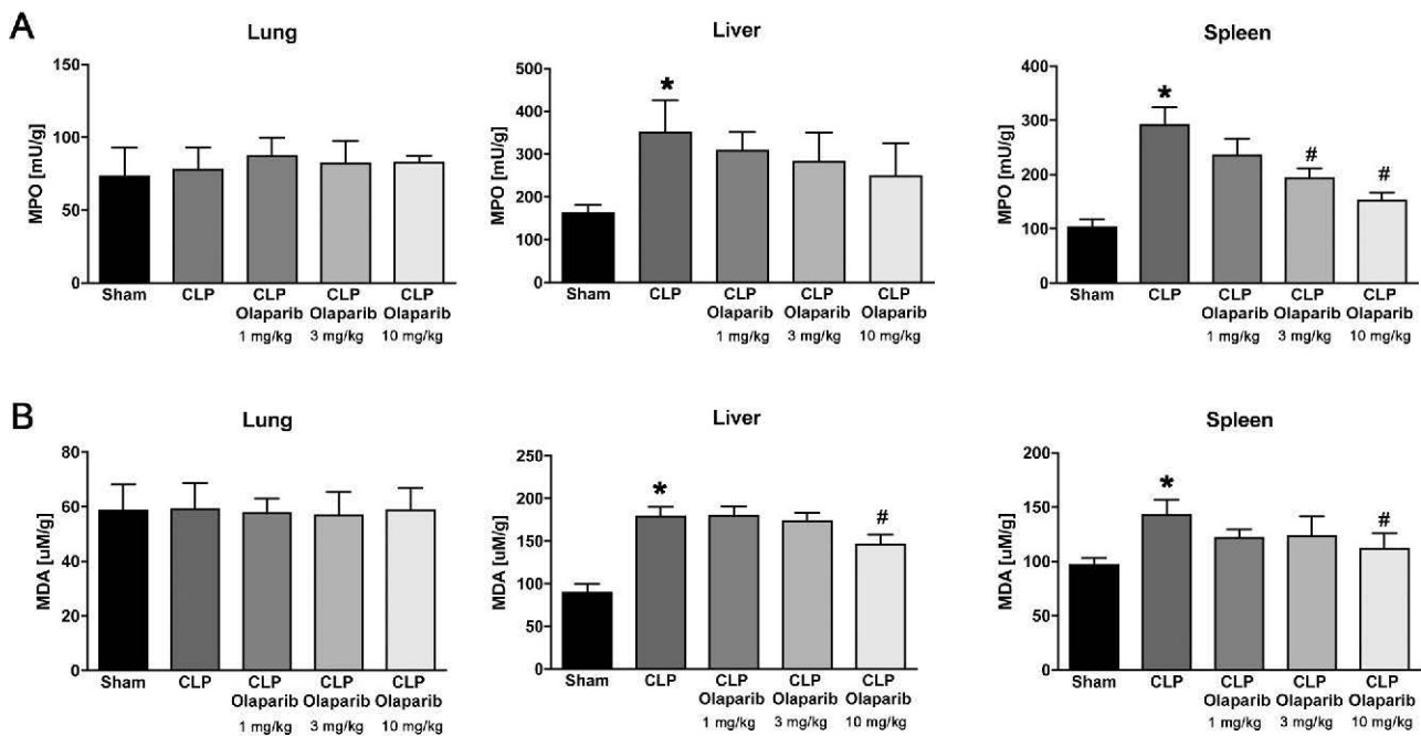
Fig. 1. Effect of olaparib on lung, liver and spleen MPO and MDA levels in young male Balb/c mice subjected to CLP. (A): Lung, liver and spleen MPO levels (expressed as milliunits [mU]/gram tissue) and (B): lung, liver and spleen MDA levels (expressed as µM/gram tissue) are shown in sham mice (not subjected to CLP) ("Sham"), in vehicle-treated mice subjected to CLP for 24 h ("CLP") and in mice subjected to CLP in the presence of various doses of olaparib ("CLP Olaparib 1 mg/kg", "CLP Olaparib 3 mg/kg" and "CLP Olaparib 10 mg/kg"). Data are shown as mean \pm SEM of 10 animals for each group; *p < 0.05 shows significant increase in MPO in response to CLP, compared to the sham group; #p < 0.05 shows significant protective effect of olaparib in CLP mice compared to vehicle-treated CLP mice.
