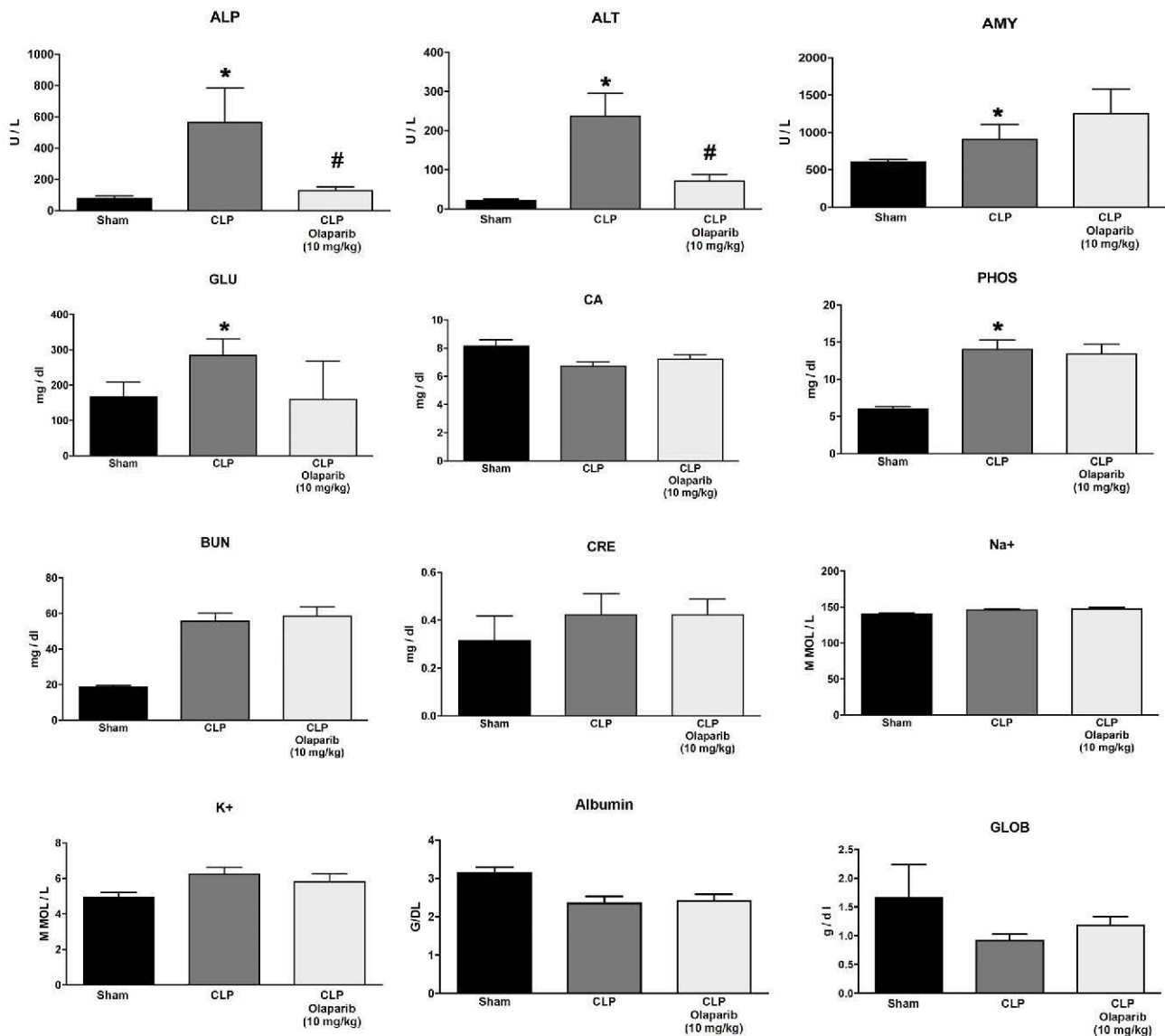
Fig. 21. Effect of olaparib on selected parameters of organ injury in aged female Balb/c mice subjected to CLP. Various physiological and organ injury marker levels: alkaline phosphatase (ALP), alanine aminotransferase (ALT), amylase (AMY), plasma glucose (GLU), plasma calcium ( CA^{++} ), plasma phosphate (PHOS), plasma blood urea nitrogen (BUN), plasma creatinine (CRE), plasma sodium ( Na^+ ), plasma potassium ( Na^+ ), plasma albumin (ALB) and plasma globulin (GLOB) measured by Vetscan analysis, are shown in sham mice (not subjected to CLP) ("Sham"), in vehicle-treated mice subjected to CLP for 24 h ("CLP") and in mice subjected to CLP in the presence of various doses of olaparib ("CLP Olaparib 1 mg/kg", "CLP Olaparib 3 mg/kg" and "CLP Olaparib 10 mg/kg"). Data are shown as mean \pm SEM of 10 animals for each group; * p < 0.05 shows significant increase in the respective parameter in response to CLP, compared to the sham group; # p < 0.05 shows significant effect of olaparib in CLP mice (compared to vehicle-treated CLP mice).
