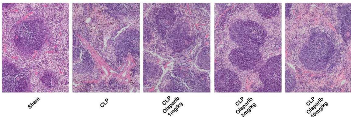
Fig. 5. Effect of olaparib on histological alterations injury in the spleen of young male Balb/c mice subjected to CLP. Representative histological pictures are shown in sham mice (not subjected to CLP) ("Sham"), in vehicle-treated mice subjected to CLP for 24 h ("CLP") and in mice subjected to CLP in the presence of various doses of olaparib ("CLP Olaparib 1 mg/kg", "CLP Olaparib 3 mg/kg" and "CLP Olaparib 10 mg/kg"). Pictures are selected from n = 5 animals for each group.
