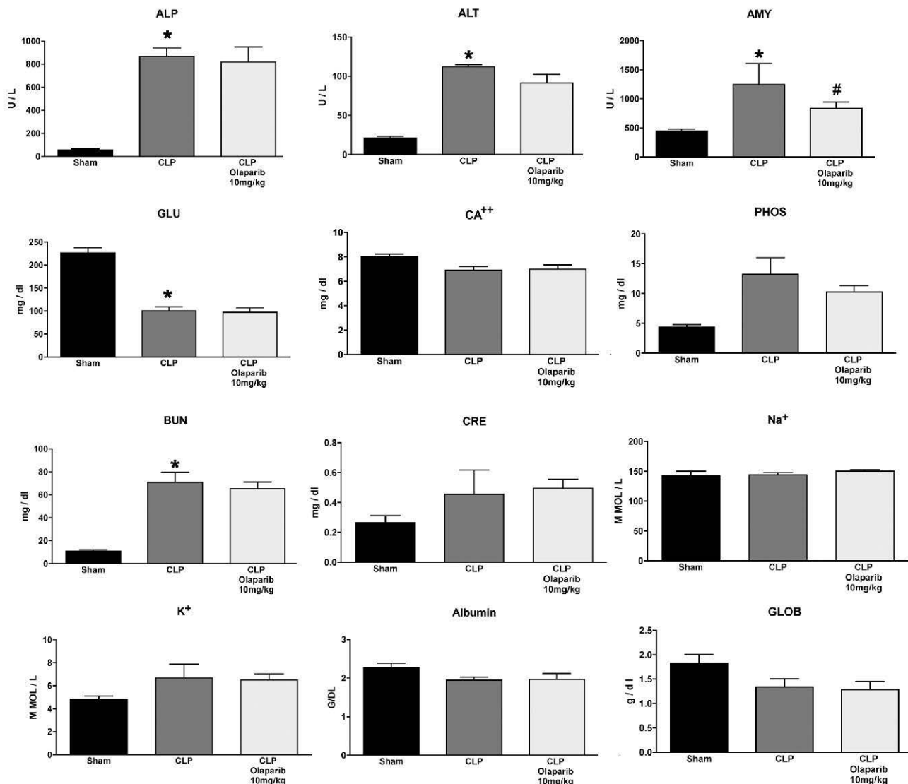
Fig. 19. Effect of olaparib on selected parameters of organ injury in aged male Balb/c mice subjected to CLP. Various physiological and organ injury marker levels: alkaline phosphatase (ALP), alanine aminotransferase (ALT), amylase (AMY), plasma glucose (GLU), plasma calcium (CA ++ ), plasma phosphate (PHOS), plasma blood urea nitrogen (BUN), plasma creatinine (CRE), plasma sodium (Na + ), plasma potassium (K + ), plasma albumin (ALB) and plasma globulin (GLOB) measured by Vetscan analysis, are shown in sham mice (not subjected to CLP) ("Sham"), in vehicle-treated mice subjected to CLP for 24 h ("CLP") and in mice subjected to CLP in the presence of various doses of olaparib ("CLP Olaparib 1 mg/kg", "CLP Olaparib 3 mg/kg" and "CLP Olaparib 10 mg/kg"). Data are shown as mean \pm SEM of 10 animals for each group; *p < 0.05 shows significant increase in the respective parameter in response to CLP, compared to the sham group; #p < 0.05 shows significant effect of olaparib in CLP mice (compared to vehicle-treated CLP mice).
