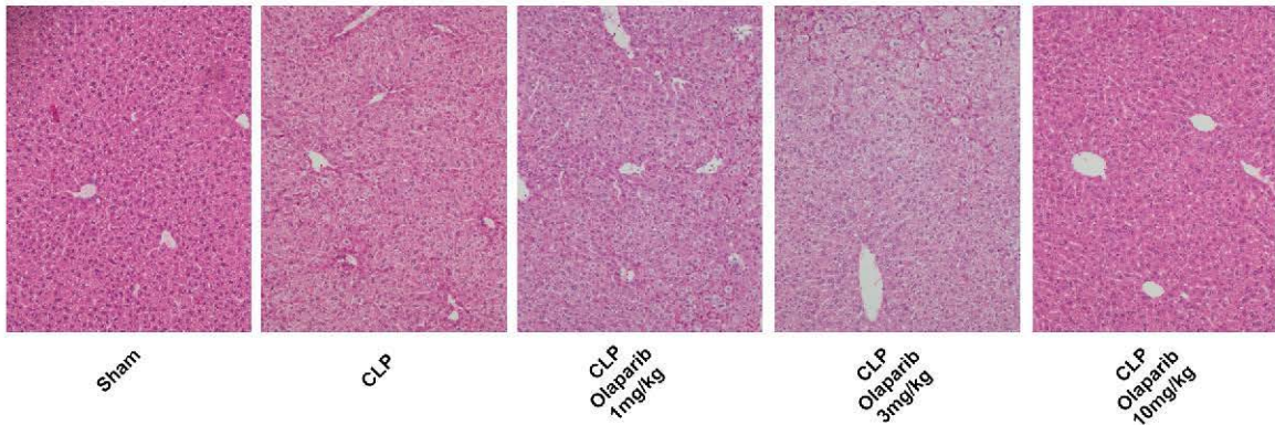
Fig. 4. Effect of olaparib on histological alterations injury in the liver of young male Balb/c mice subjected to CLP. Representative histological pictures are shown in sham mice (not subjected to CLP) ("Sham"), in vehicle-treated mice subjected to CLP for 24 h ("CLP") and in mice subjected to CLP in the presence of various doses of olaparib ("CLP Olaparib 1 mg/kg", "CLP Olaparib 3 mg/kg" and "CLP Olaparib 10 mg/kg"). Pictures are selected from n = 5 animals for each group.
