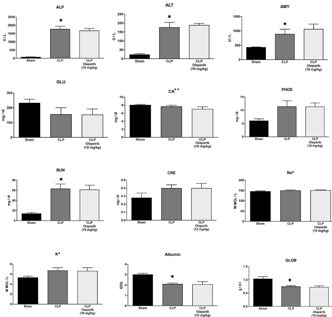
Fig. 17. Effect of olaparib on selected parameters of organ injury in young female Balb/c mice subjected to CLP. Various physiological and organ injury marker levels: alkaline phosphatase (ALP), alanine aminotransferase (ALT), amylase (AMY), plasma glucose (GLU), plasma calcium ( Ca^{++} ), plasma phosphate (PHOS), plasma blood urea nitrogen (BUN), plasma creatinine (CRE), plasma sodium ( Na^+ ), plasma potassium ( K^+ ), plasma albumin (ALB) and plasma globulin (GLOB) measured by Vetscan analysis, are shown in sham mice (not subjected to CLP) ("Sham"), in vehicle-treated mice subjected to CLP for 24 h ("CLP") and in mice subjected to CLP in the presence of various doses of olaparib ("CLP Olaparib 1 mg/kg", CLP Olaparib 3 mg/kg and "CLP Olaparib 10 mg/kg"). Data are shown as mean \pm SEM of 10 animals for each group; *p < 0.05 shows significant increase in the respective parameter in response to CLP, compared to the sham group.
