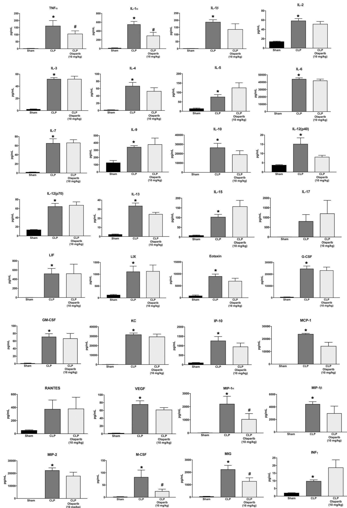
Fig. 22. Effect of olaparib on the levels of various circulating mediators (cytokines, chemokines, growth factors) in aged female Balb/c mice subjected to CLP. Values are shown in sham mice (not subjected to CLP) ("Sham"), in vehicle-treated mice subjected to CLP for 24 h ("CLP") and in mice subjected to CLP in the presence of 10 mg/kg olaparib ("CLP Olaparib 10 mg/kg"). Data are shown as mean \pm SEM of 10 animals for each group; * p < 0.05 shows significant increase in the respective parameter in response to CLP, compared to the sham group; # p < 0.05 shows significant protective effect of olaparib in CLP mice compared to vehicle-treated CLP mice.
