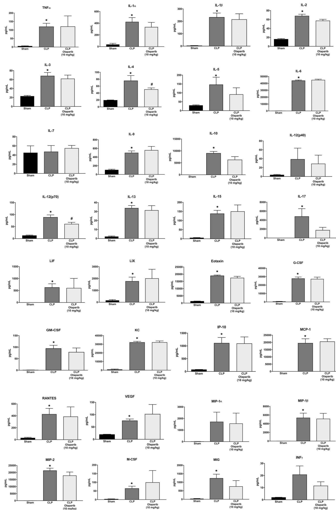
Fig. 20. Effect of olaparib on the levels of various circulating mediators (cytokines, chemokines, growth factors) in aged male Balb/c mice subjected to CLP. Values are shown in sham mice (not subjected to CLP) ("Sham"), in vehicle-treated mice subjected to CLP for 24 h ("CLP") and in mice subjected to CLP in the presence of 10 mg/kg olaparib ("CLP Olaparib 10 mg/kg"). Data are shown as mean \pm SEM of 10 animals for each group; * p < 0.05 shows significant increase in the respective parameter in response to CLP, compared to the sham group; # p < 0.05 shows significant protective effect of olaparib in CLP mice compared to vehicle-treated CLP mice.
