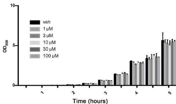
Fig. 9. Effect of olaparib on E. coli bacterial growth in vitro . Data show bacterial numbers at various time points in vehicle-treated group, and in the groups of bacteria in the presence of various concentrations (1, 3, 10, 30, 100 \mu M) olaparib for various time points (1–5 h). Data are shown as mean \pm SEM of 5 determinations per group.
