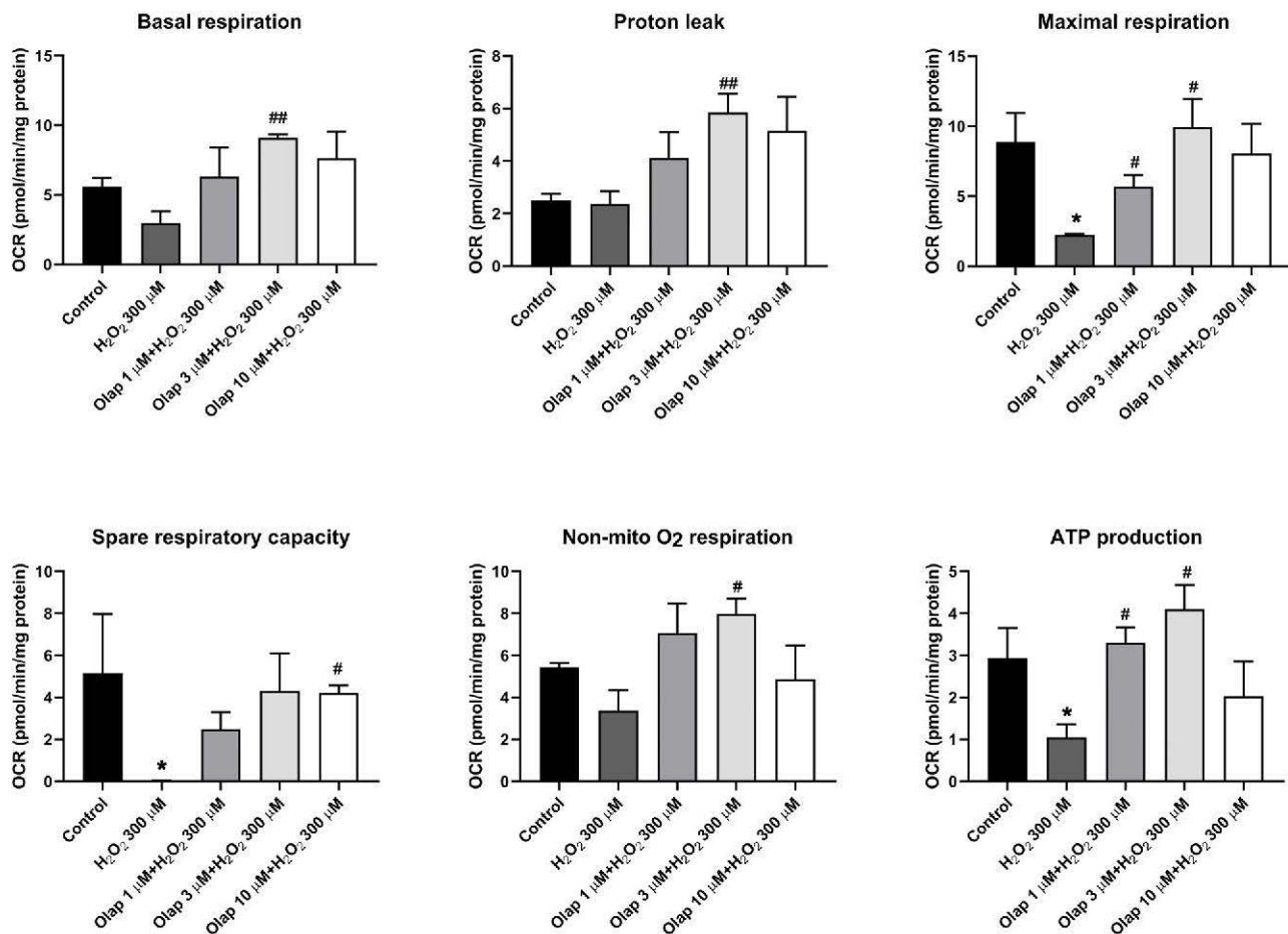
Fig. 27. Effect of olaparib on oxidative phosphorylation-related bioenergetic parameters in U937 cells subjected to H 2 O 2 -induced oxidative stress in vitro . Results are shown in control cells, in H 2 O 2 (300 μM) treated cells at 1 h, and in H 2 O 2 (300 μM) treated cells at 1 h in the presence of pretreatment with 1, 3 or 10 μM olaparib. Results are indicated as mean ± SEM of n = 3 per condition. *p < 0.05 shows a significant change in response to H 2 O 2 , compared to control cells; #p < 0.05 and ##p < 0.01 show significant protective effect of olaparib in H 2 O 2 challenged cells compared to vehicle-treated H 2 O 2 challenged cells.
