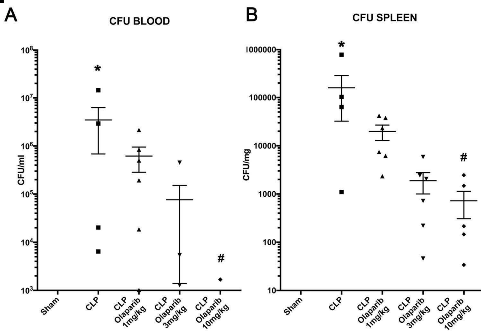
Fig. 8. Effect of olaparib on blood and spleen bacterial colony-forming unit (CFU) numbers in young male Balb/c mice subjected to CLP. (A): Blood CFUs (expressed as CFU/ml) and (B) spleen CFUs (expressed as CFU/mg) are shown in sham mice (not subjected to CLP) ("Sham"), in vehicle-treated mice subjected to CLP for 24 h ("CLP") and in mice subjected to CLP in the presence of various doses of olaparib ("CLP Olaparib 1 mg/kg", CLP Olaparib 3 mg/kg" and "CLP Olaparib 10 mg/kg"). Data are shown as mean \pm SEM of 10 animals for each group; * p < 0.05 shows significant increases in CFUs in response to CLP, compared to the sham group; # p < 0.05 shows significant effect of olaparib on CFU values in CLP mice compared to vehicle-treated CLP mice.
