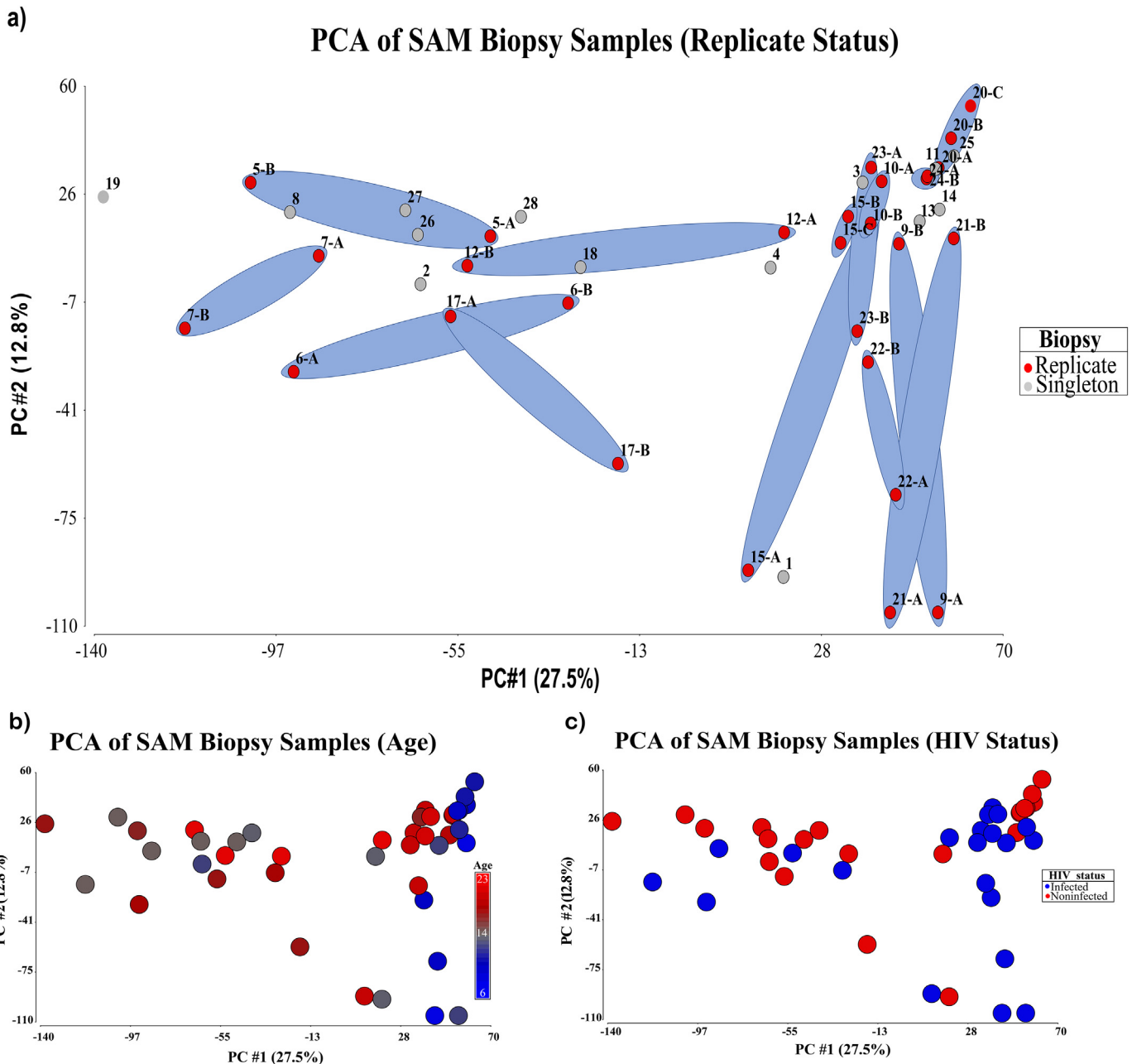
Fig. 1. Principal Component Analysis of transcriptomes of Zambian children with Severe Acute Malnutrition. (A) pairs of duplicate biopsies from the same child, taken on the same day, are ringed; only one pair shows a difference in both components between biopsies from the same child. (B) the influence of age on transcriptomes. (C) the influence of HIV on the transcriptome, showing no discernible pattern.
