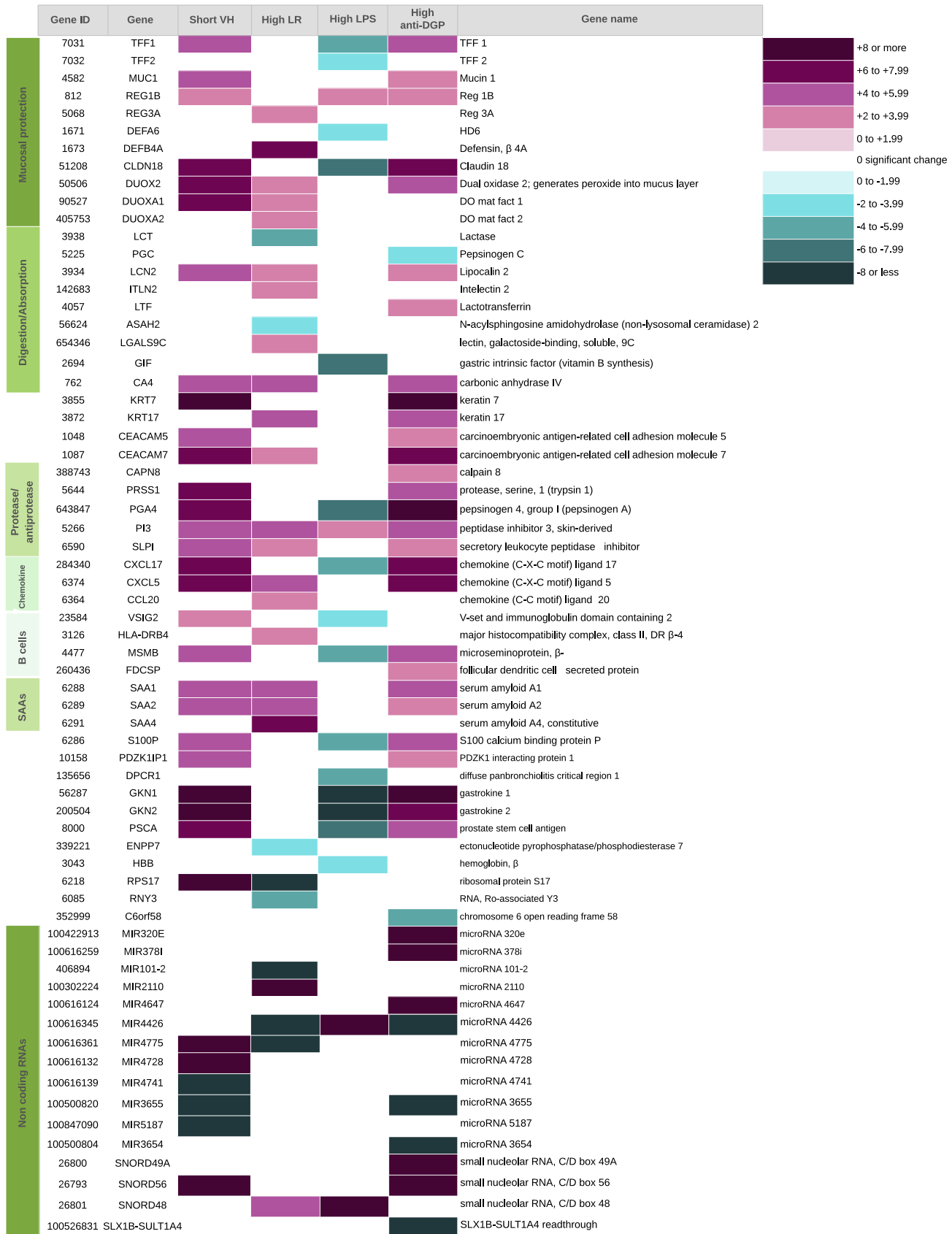
Fig. 2. Differentially expressed genes identified by NOIsq analysis. Heat map of 66 differentially expressed. Colours represent the log 2 fold change in more severe enteropathy (short villi, high lactulose permeation, high plasma lipopolysaccharide, and higher blood anti-deamidated gliadin peptide concentration).
