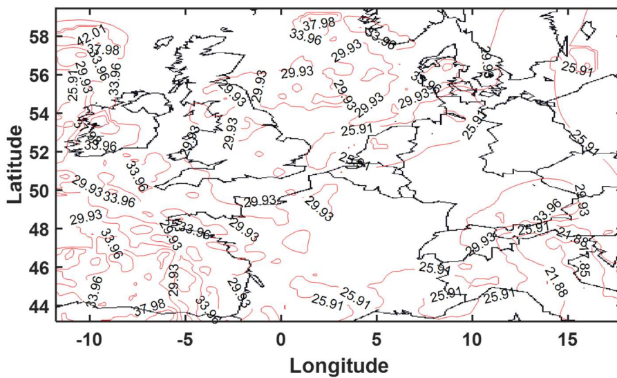
Figure 10: Contour map of 0.01% exceeded rain rates for an average year given by ITU-R P837-
