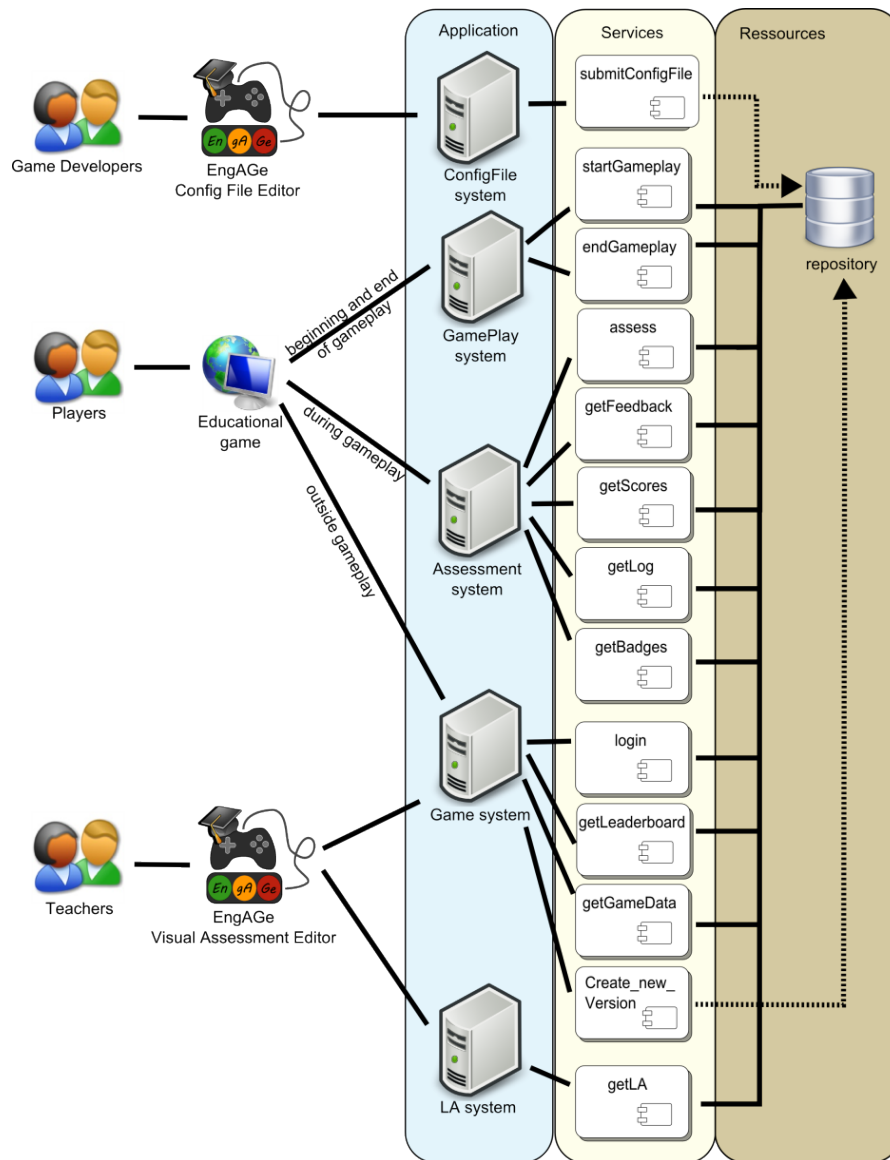
Figure 8: Overview Architecture of EngAGE
