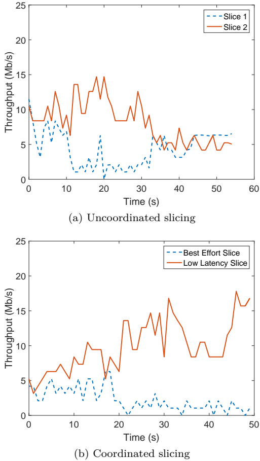
Fig. 9: Mobile network slicing.
