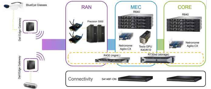
Fig. 7: 5G eHealth prototyping - hardware stack.
