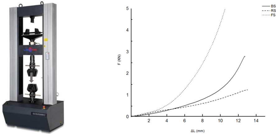
Fig. 2. The elastic modulus test system (left). \Delta L represented the deformation of the materials after compressing, and F represented the force to press the materials.
