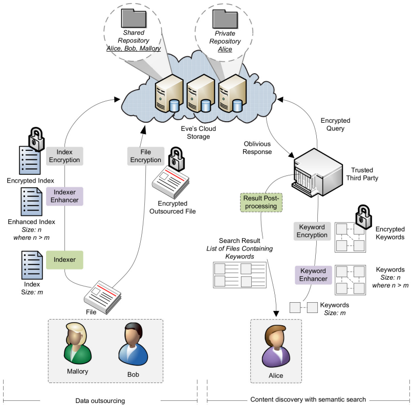
Fig 2. Semantic search over encrypted data - conceptual model
