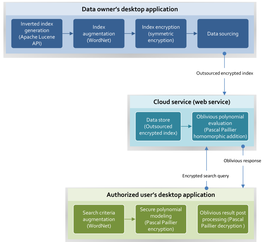
Fig 5. Core functionalities - desktop application and web service.
