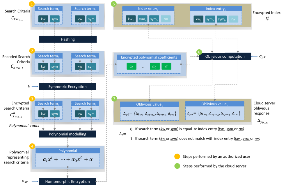
Fig 4. Encoding semantically enriched search criteria and modeling search query for oblivious computation.
