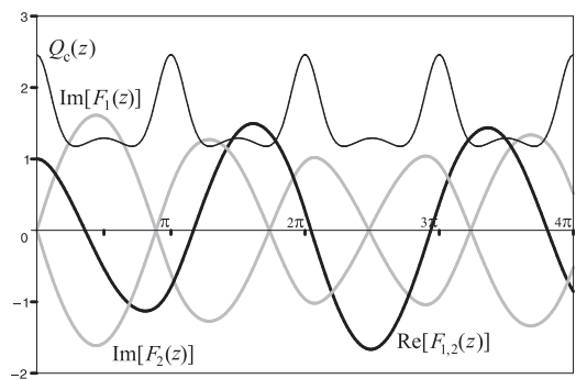
Fig. 7. Floquet-Bloch waves F_1(z) and F_2(z) in the allowed band of the Casperson potential Q_c(z) (black line) for q = -0.25 and a = 1.20 . The real parts, \Re[F_1(z)] = \Re[F_2(z)] , are shown by a thick black line and imaginary parts, \Im[F_2(z)] = -\Im[F_1(z)] , are shown by thick grey lines. Note that \Re[F_{1,2}(z)] = u(z) .
