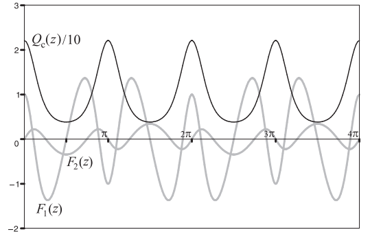
Fig. 13. Periodic Floquet-Bloch waves F_1(z) and F_2(z) in the third incipient band ( m = 3 ) of the Casperson potential for q = -0.25 .
