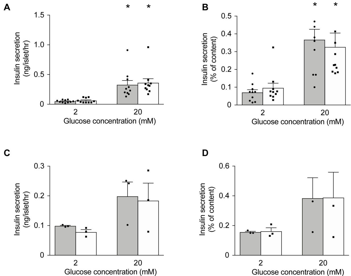
Fig 1. Acute lowering of Mg^{2+} does not affect insulin secretion in pancreatic \beta cells under normal- and hyperglycemic conditions. (A-B) Insulin secretion from isolated islets ( n = 10 replicates, islets from 16 mice, 8 islets per replicate) challenged by 2 mM and 20 mM glucose at 0.5 mM Mg^{2+} (solid bar) and 1.0 mM Mg^{2+} (open bar) for 1 hr, after 24 hrs of culture at 11 mM glucose (1.2 mM Mg^{2+} ). (C-D) Insulin secretion from mouse pancreatic islets ( n = 3 , islets from 3 mice, 8 islets per replicate) stimulated by 2 mM and 20 mM glucose with 0.5 mM Mg^{2+} (solid bar) and 1.0 mM Mg^{2+} (open bar) for 1 hr after 24 hrs of culture at 25 mM glucose (1.2 mM Mg^{2+} ). Insulin secretion is presented as ng/islet/hr (A, C) and as normalized to total insulin content (B, D). Statistical significance was determined by two-way ANOVA. *, p < 0.05 , 20 mM glucose vs. 2 mM glucose.
