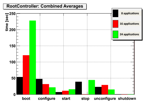
(b) FSM transition times for an RC tree controlling 30 nodes with 8, 16 or 24 applications.
