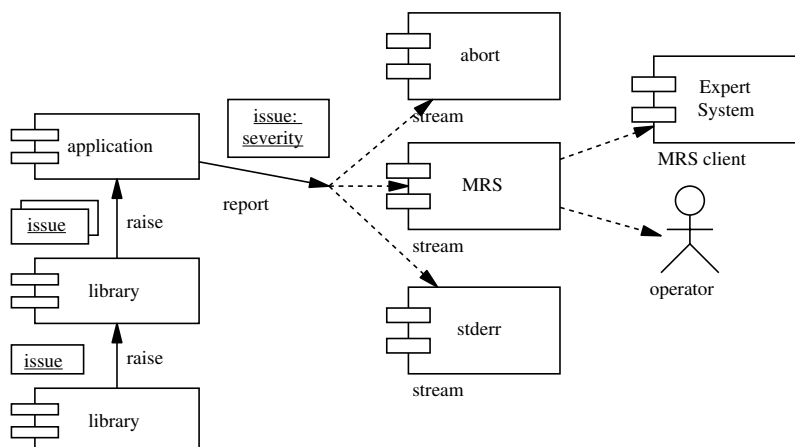
Figure 9. Flow of ERS issues. A library creates an issue as a C++ exception and passes it to a higher level. Finally an application assigns a severity to the issue and reports it to one or more streams.
