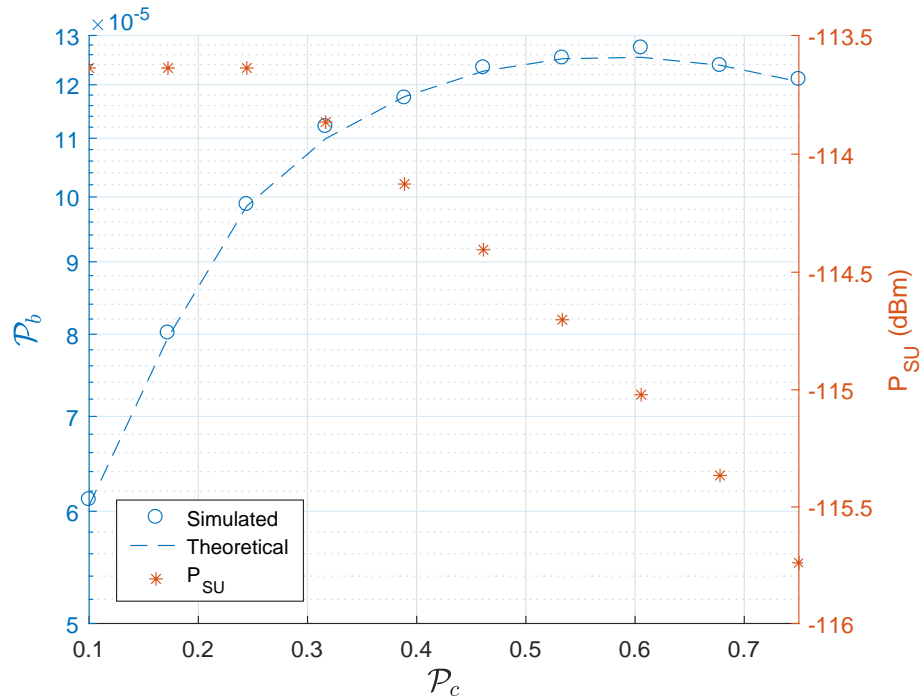
Figure 23. PU performance with a fixed SU value \mathcal{P}_d = 0.25 and a range of SU (\mathcal{P}_c, P_{SU}) operating pairs on the linear boundary.
