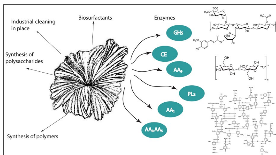
FIGURE 1 Biotechnological applications of Schizophyllum commune . Glycoside hydrolase (GH), carbohydrate esterase (CE), glycosyltransferase (GT), polysaccharide lyase (PL), lytic polysaccharide monooxygenase (AA9), laccase (AA1), peroxide-producing enzymes (AA3, and AA5)
