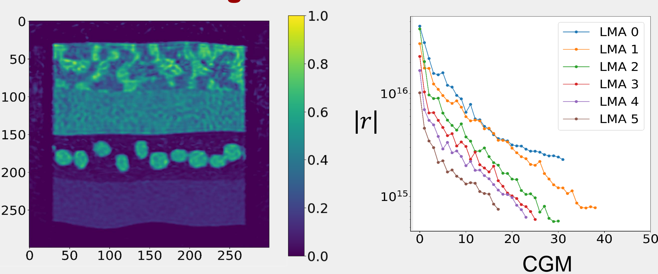
Figure 2: On the left, single-scale reconstruction from the complete diffraction data-set with zero-valued input is shown; on the right, residual values over LMA and CGM iterations are shown.
