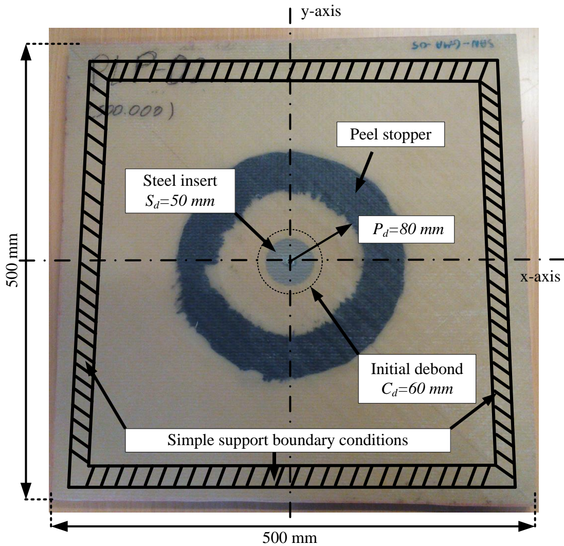
Figure 1. Layout and dimensions of foam cored sandwich panel test specimens with embedded PU peel stopper.
