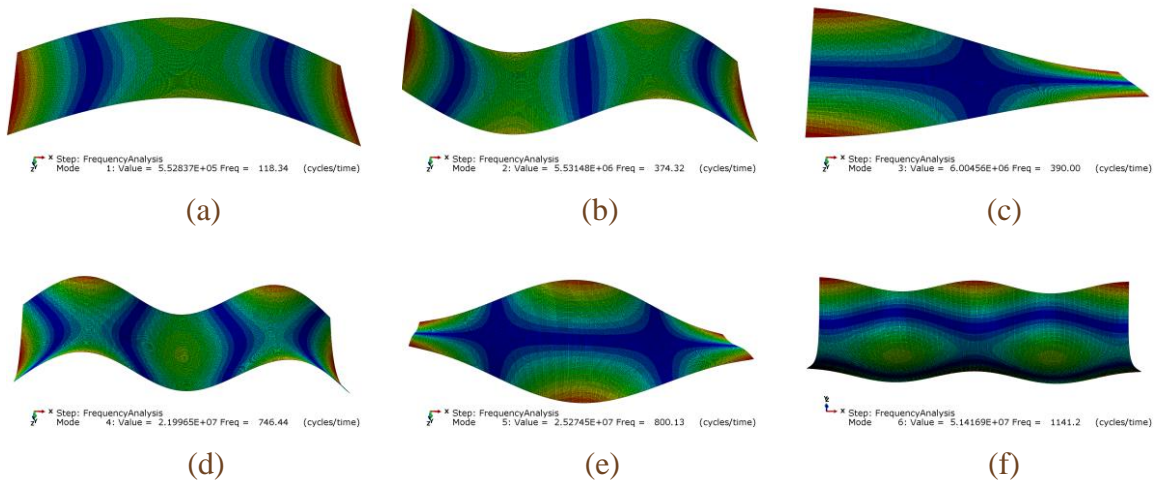
Figure 5: Mode shapes of the (a)-(f) first-sixth non-rigid FE modes
