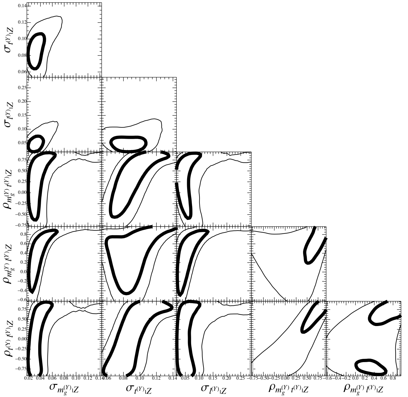
Fig. B.4. Probability distributions of the scatter parameters from the multi-response regression. The thick (thin) contours include the 1-(2-) \sigma confidence region in two dimensions, here defined as the region within which the probability is larger than \exp[-2.3/2] ( \exp[-6.17/2] ) of the maximum.
