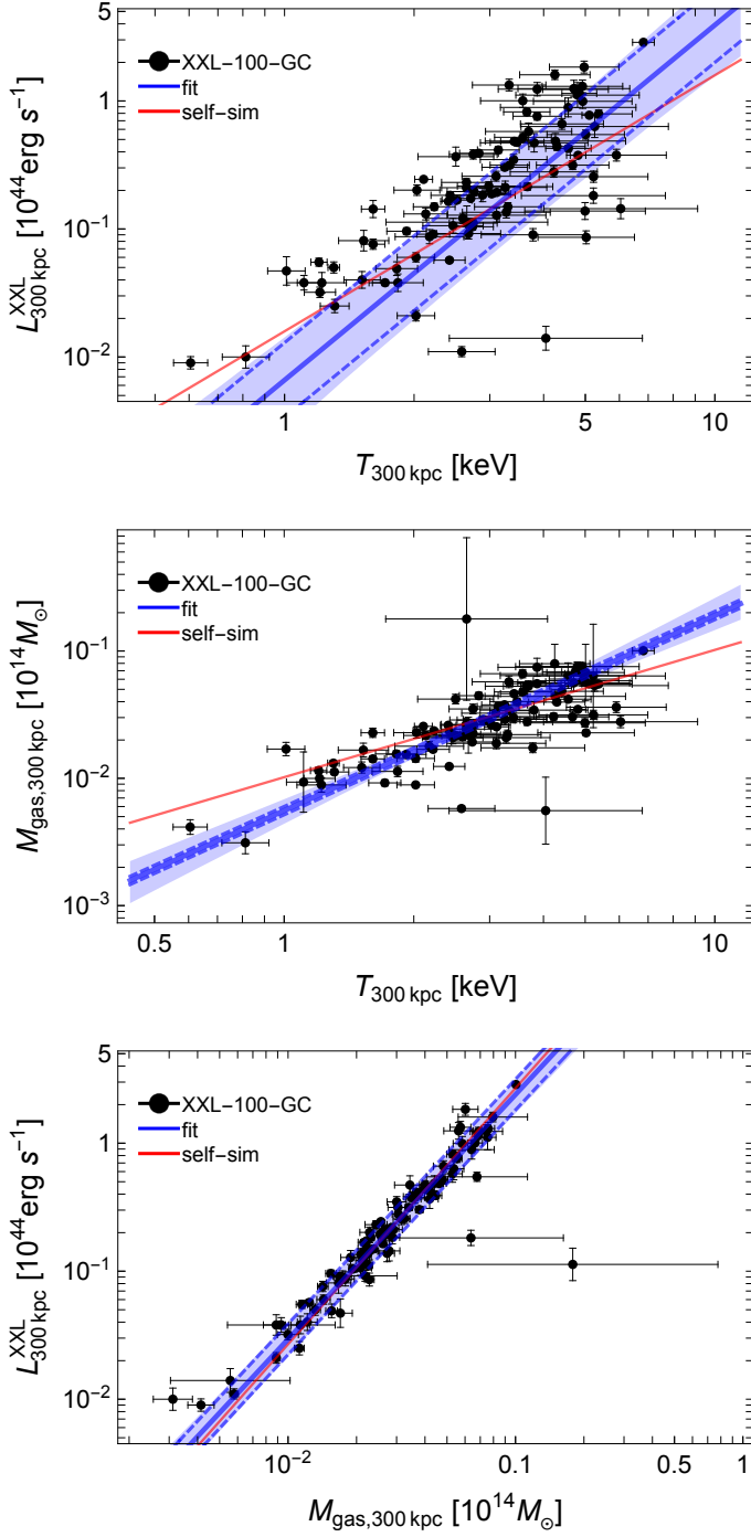
Fig. 2. Scaling relations. The black points mark the data, the blue lines represent the fitted scaling relation at the median redshift. The dashed blue lines show the median scaling relation (full blue line) plus or minus the intrinsic scatter \sigma_{YZ} . The shaded blue region encloses the 68.3 per cent confidence region around the median due to uncertainties on the scaling parameters. The red line shows the self-similar prediction. Top panel: scaling between luminosity and temperature, l-t . Middle panel: scaling between gas mass and temperature, m_g-t . Bottom panel: scaling between luminosity and gas mass, l-m_g .
