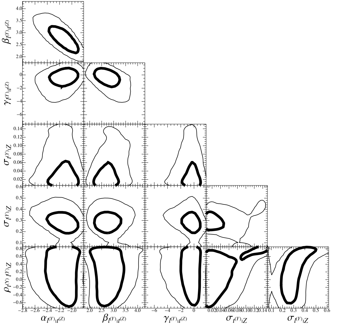
Fig. B.1. Probability distributions of the parameters of the scaling relation between luminosity and temperature, l-t . The thick (thin) lines include the 1-(2)- \sigma confidence region in two dimensions, here defined as the region within which the probability is larger than \exp[-2.3/2] ( \exp[-6.17/2] ) of the maximum.
