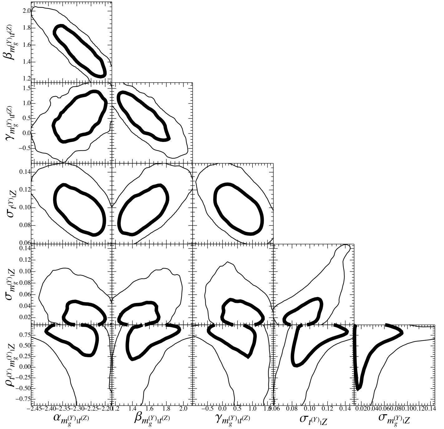
Fig. B.2. Probability distributions of the parameters of the scaling relation between gas mass and temperature, m_g - t . The thick (thin) contours include the 1-(2)- \sigma confidence region in two dimensions, here defined as the region within which the probability is larger than \exp[-2.3/2] ( \exp[-6.17/2] ) of the maximum.
