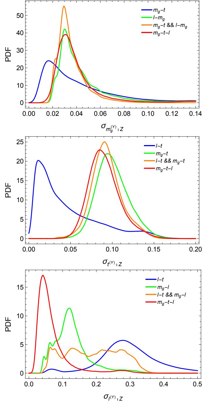
Fig. 3. Inferred probability density functions of the conditional intrinsic scatters with respect to the mass substitute. The blue and the green lines show the results based on the fits of pairs; the orange and the red lines show the densities obtained with the joint analysis of pair fits or with the multi-response regression, respectively. Top panel: gas mass intrinsic scatter. Middle panel: temperature intrinsic scatter. Bottom panel: luminosity intrinsic scatter.
