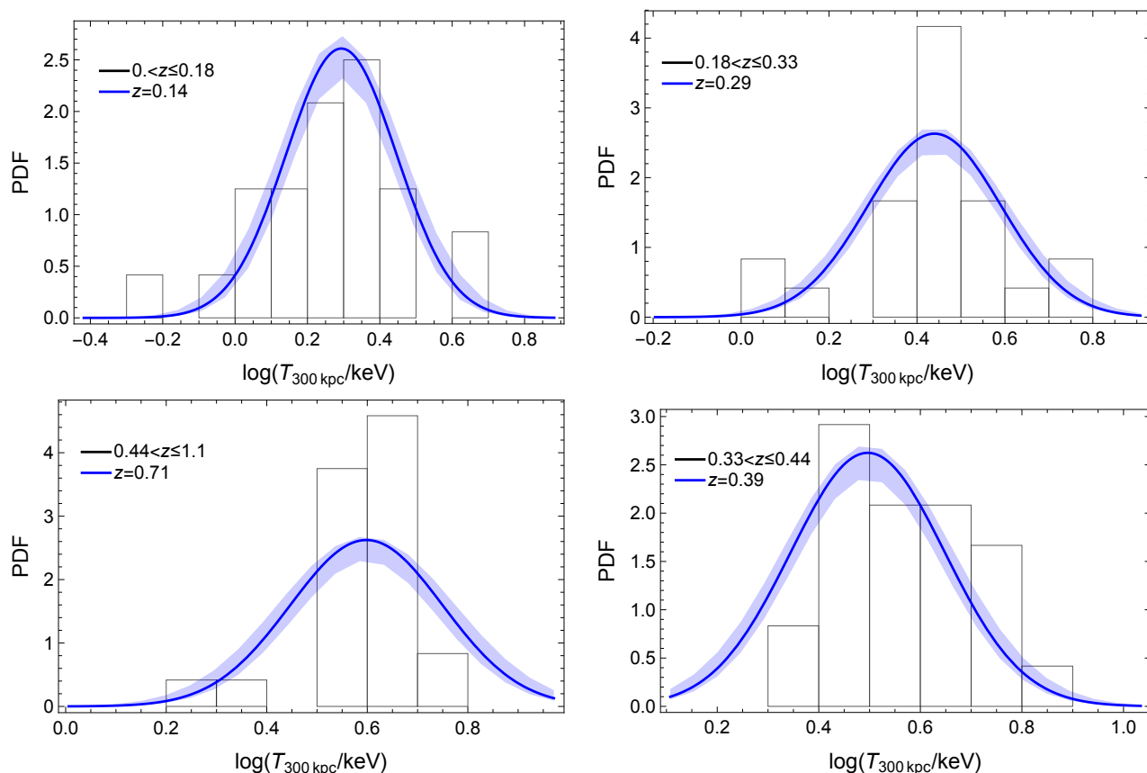
Fig. 5. Temperature function of the clusters from the l - t analysis in four redshift bins. The black histogram groups the observed temperatures. The blue line is the normal approximation estimated from the regression at the median redshift in the bin. The shaded blue region encloses the 68.3 per cent probability region around the median relation due to uncertainties on the parameters. The function for the observed temperatures is estimated from the regression output, i.e. the function of the unscattered temperatures, by smoothing the prediction with a Gaussian whose variance is given by the quadratic sum of the intrinsic scatter of the (logarithmic) temperature with respect to the unscattered temperature and the median observational uncertainty. Redshift increases clockwise from the top left to the bottom left panel. The median and the boundaries of the redshift bins are indicated in the legends of the respective panels.
