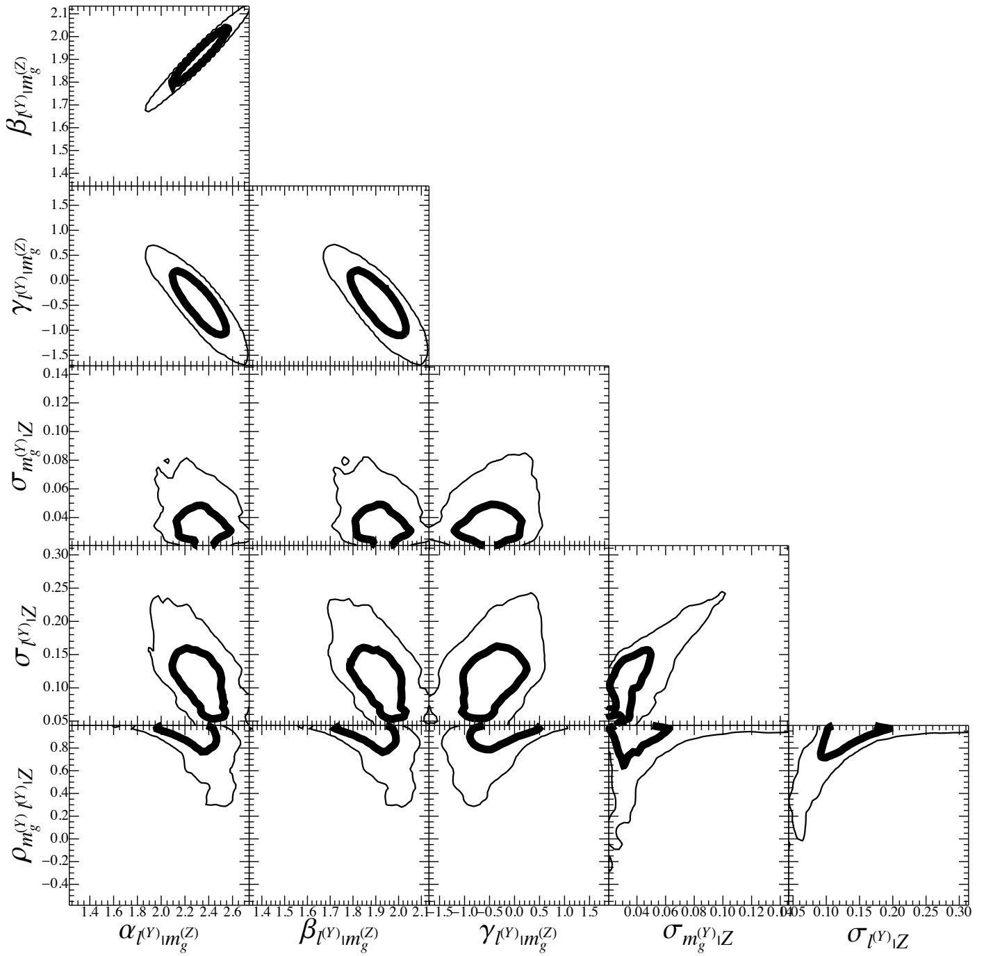
Fig. B.3. Probability distributions of the parameters of the scaling relation between luminosity and gas mass, l - m_g . The thick (thin) contours include the 1-(2)- \sigma confidence region in two dimensions, here defined as the region within which the probability is larger than \exp[-2.3/2] ( \exp[-6.17/2] ) of the maximum.
