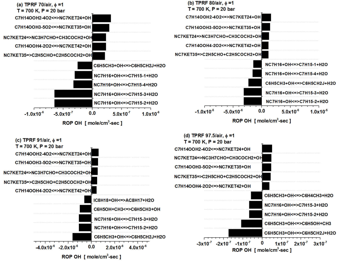
Figure 9: ROP analyses of \dot{\text{O}}\text{H} radical at T = 700 \text{ K} , p = 20 \text{ bar} , \phi = 1 ; (a) TPRF 70/air, (b) TPRF 80/air, (c) TPRF 91/air, and (d) TPRF 97.5/air mixtures. LLNL mech [39] is used for ROP analyses. The ROP analyses are conducted at a time corresponding to two-thirds of the exponential growth of \dot{\text{O}}\text{H} radical concentration
