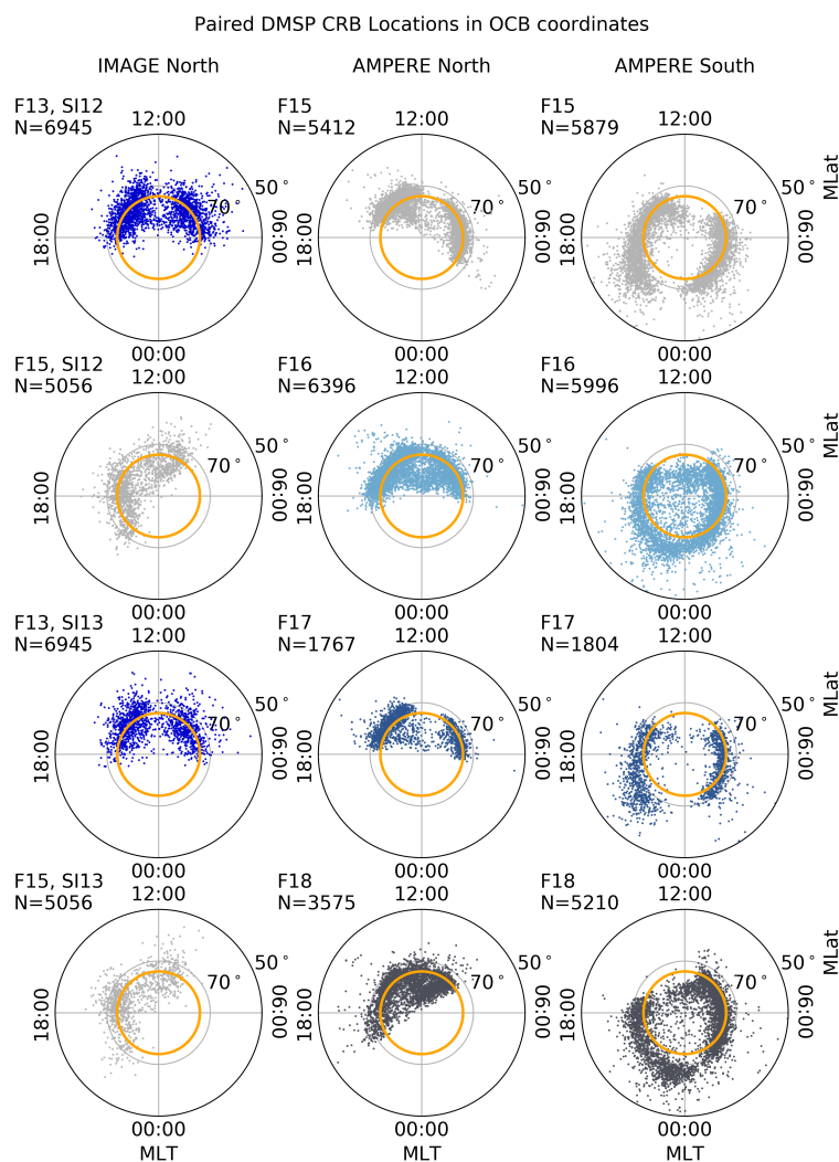
Figure 4. Paired IMAGE and AMPERE OCBs with DMSP CRBs for the available hemispheres and each satellite. The IMAGE data shows the SI-12 and SI-13 observations for the northern hemisphere (left column), while the median elliptical correction was applied to obtain the AMPERE OCBs shown in the middle and right columns (which show the northern and southern hemispheres, respectively). The scattered points show the DMSP IVM CRBs, while the gold circle shows the IMAGE or AMPERE OCB. To simplify the comparison, the DMSP IVM CRB locations are plotted in adjusted polar coordinates (Burrell and Chisham, 2018).
