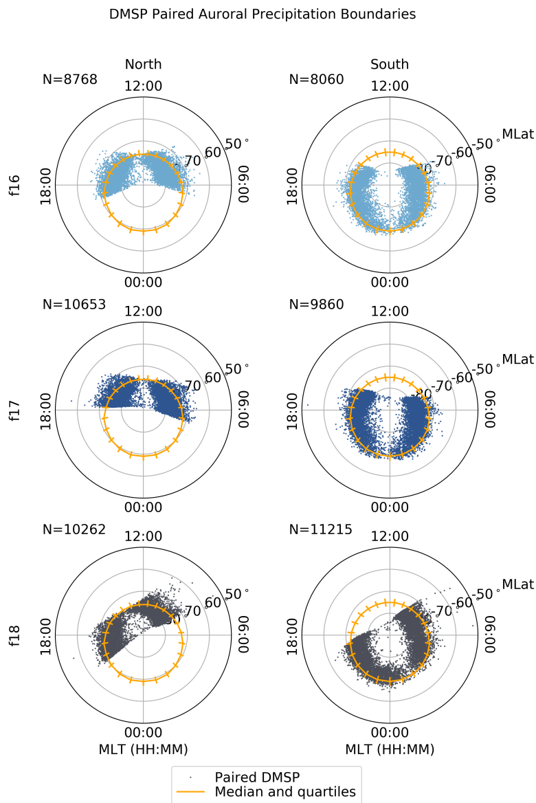
Figure 1. Paired AMPERE R1/R2 boundaries and DMSP SSJ OCBs for both hemispheres (northern in the left column and southern in the right column) and each satellite. The scattered points show the DMSP SSJ OCBs, while the gold circle shows the median location of the AMPERE R1/R2 boundaries. The scatter bars denote the quartiles of the paired AMPERE R1/R2 boundaries.
