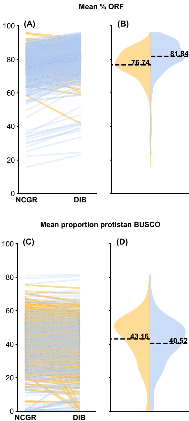
Figure 5: The percentage of contigs with a predicted ORF (A, B) and the percentage of complete protistan universal single-copy orthologs (BUSCO) recovered in each assembly (C, D). In blue (right side B, D) are the DIB re-assemblies and in yellow (left side of B, D) are the original 'nt' assemblies from NCGR. Slope graphs (A, C) compare values between the DIB and the NCGR 'nt' assemblies. Yellow lines represent negative slope values where NCGR was higher than DIB, and blue lines represent positive slope values where DIB was higher than NCGR.
