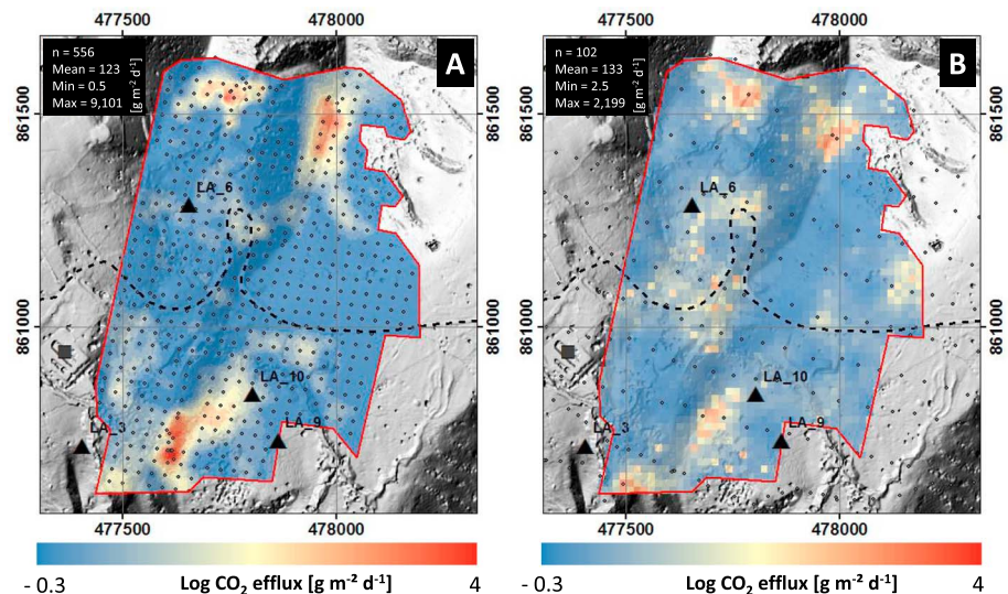
Figure 4. Detailed CO 2 efflux map from the transition zone A1 to A2 for the years 2012–2014 (a; from Hutchison et al., 2015, Hutchison, Biggs, et al., 2016) and 2016 (b). Stable degassing conditions at major degassing spots are indicated.
