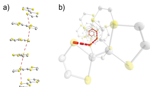
Figure 2. The helical TTF stack with a depiction of the shortest intermolecular S··S contacts (dashed red line): (a) view along the ab plane, (b) view down the c axis. Yellow and gray spheres represent S and C atoms, respectively. Phenyl rings and metal atoms were omitted for clarity.
