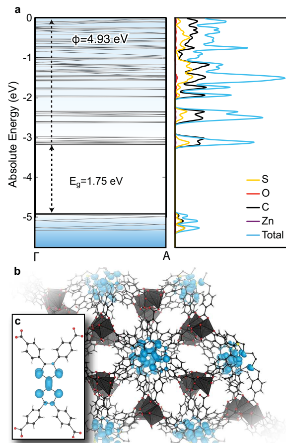
Figure 1. a) Calculated band structure and projected density of states (PDOS) of \text{Zn}_2(\text{TTFTB}) . The work function, \phi , and absolute energy scale are aligned relative to vacuum according to Ref. 20. The coordinates of the reciprocal space points are \Gamma = (0, 0, 0) and A = (0, 0, 1/2) . Corresponding pictorial representation of the valence band orbitals in \text{Zn}_2(\text{TTFTB}) (b) and one of the TTF cores (c). Zn atoms and their coordination sphere are represented by black polyhedra. Golden, red, black, and white spheres represent S, O, C, and H atoms, respectively.
