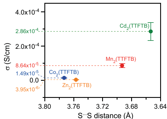
Figure 4. Correlation between S··S distance and electrical conductivity in \text{M}_2(\text{TTFTB}) .
