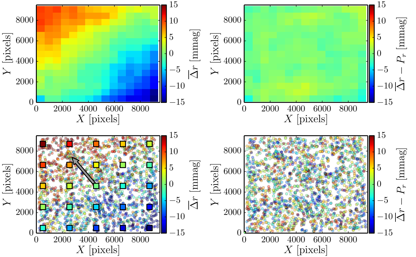
Fig. 3. Residuals of the comparison between PS1 and J-PLUS photometry in the r band, \bar{\Delta}r = \Delta r - \Delta r_{\text{atm}} , as a function of the (X, Y) position of the source on the CCD. Upper left panel: Stacked residual map of all the J-PLUS DR1 pointings. Upper right panel: Stacked residual map after applying the plane correction estimated pointing-by-pointing. Lower left panel: Residual map of the pointing p_{\text{id}} = 00315 . The gradient in the residuals of the individual sources (coloured circles) is fitted with a plane (coloured squares). The direction of maximum variation is shown with the arrow. Lower right panel: Residual map after applying the plane correction.
