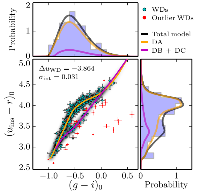
Fig. 7. Dust de-reddened (u_{\text{ims}} - r)_0 vs. (g - i)_0 colour - colour diagram of the 293 high-quality white dwarfs in J-PLUS DR1 (clean sample, cyan dots; outliers, red dots). The solid lines show the theoretical locus for DA (orange) and DB+DC WDs (magenta). The grey scale shows the most probable model that describes the observations. The upper and right blue histograms show the (g - i)_0 and (u_{\text{ims}} - r)_0 projections of the data, respectively. The projections of the total, DA, and DB+DC models are represented with the black, orange, and magenta lines. The model in all the J-PLUS colour-colour diagrams shares the parameters \mu = -0.808 , s = 0.400 , \alpha = 2.65 , f_{\text{DA}} = 0.85 , \log g = 8.01 , and \Delta C_1 = 0.007 (see text for details). The values of the filter-dependent parameters \sigma_{\text{int}} and \Delta X_{\text{WD}} are labelled in the panel.
